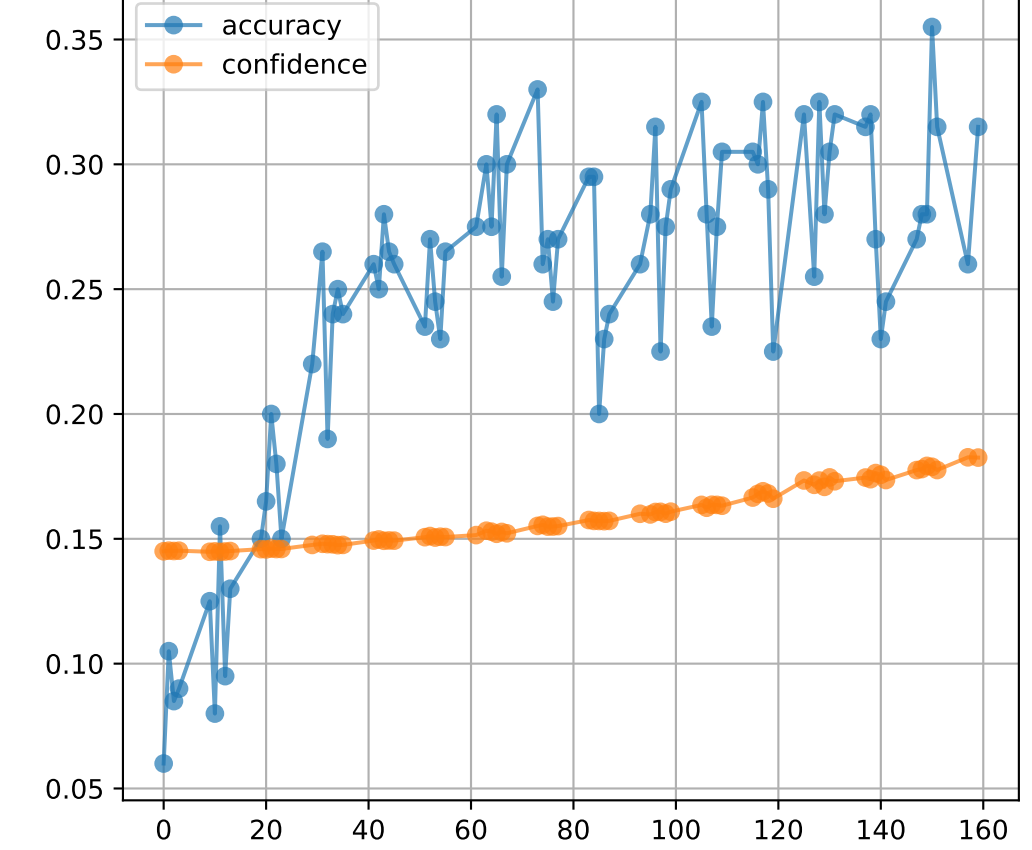
Evaluation Metrics
