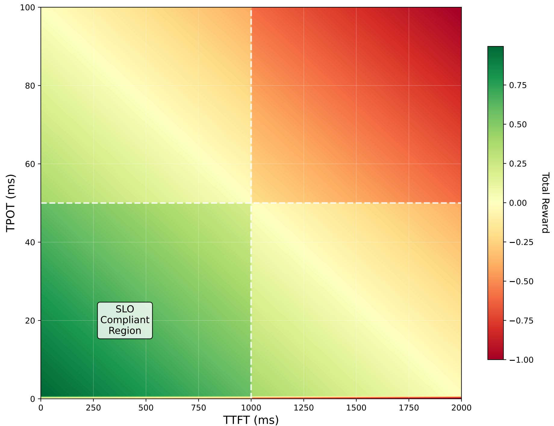
Simple Combined Reward Function Heatmap
