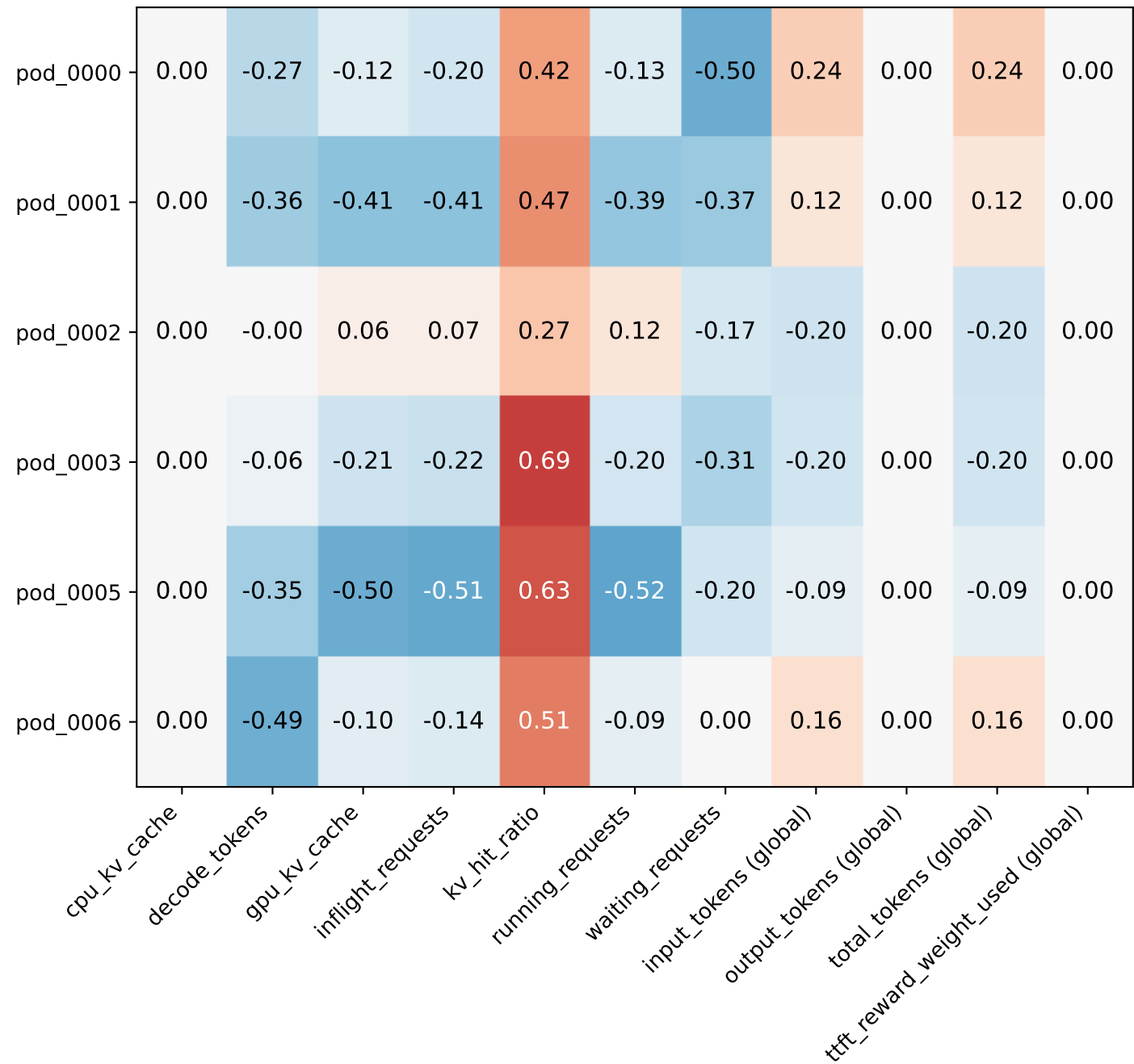
Pod State-Performance Correlations
