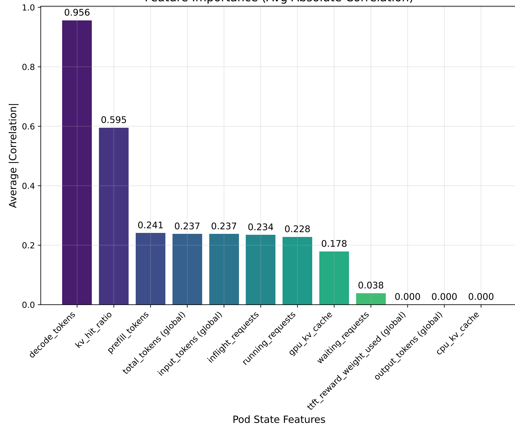
Feature Importance (Avg Absolute Correlation)
