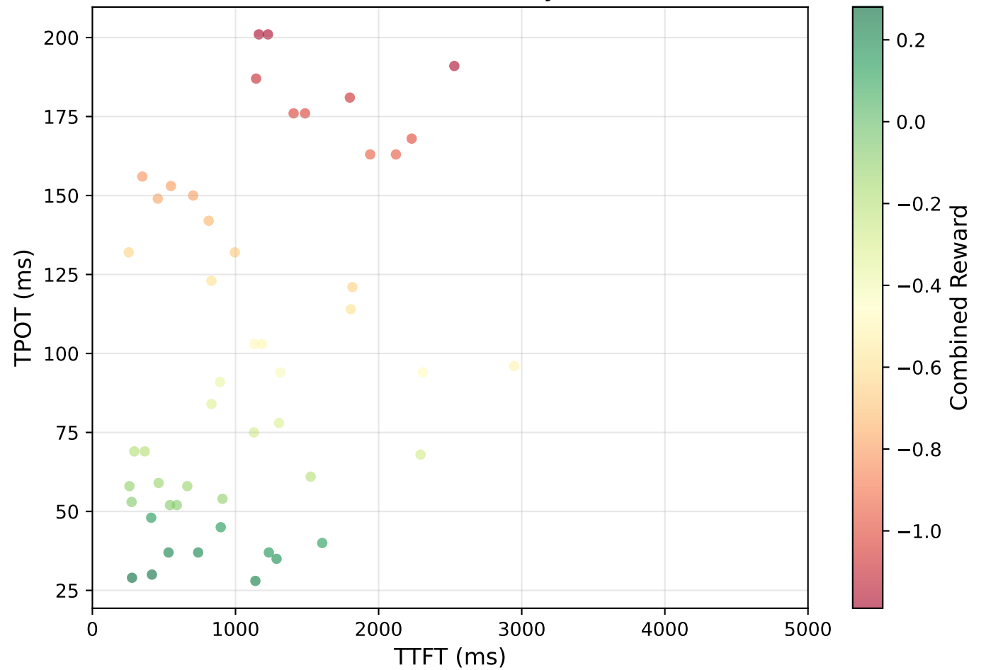
TTFT vs TPOT (colored by Reward)
