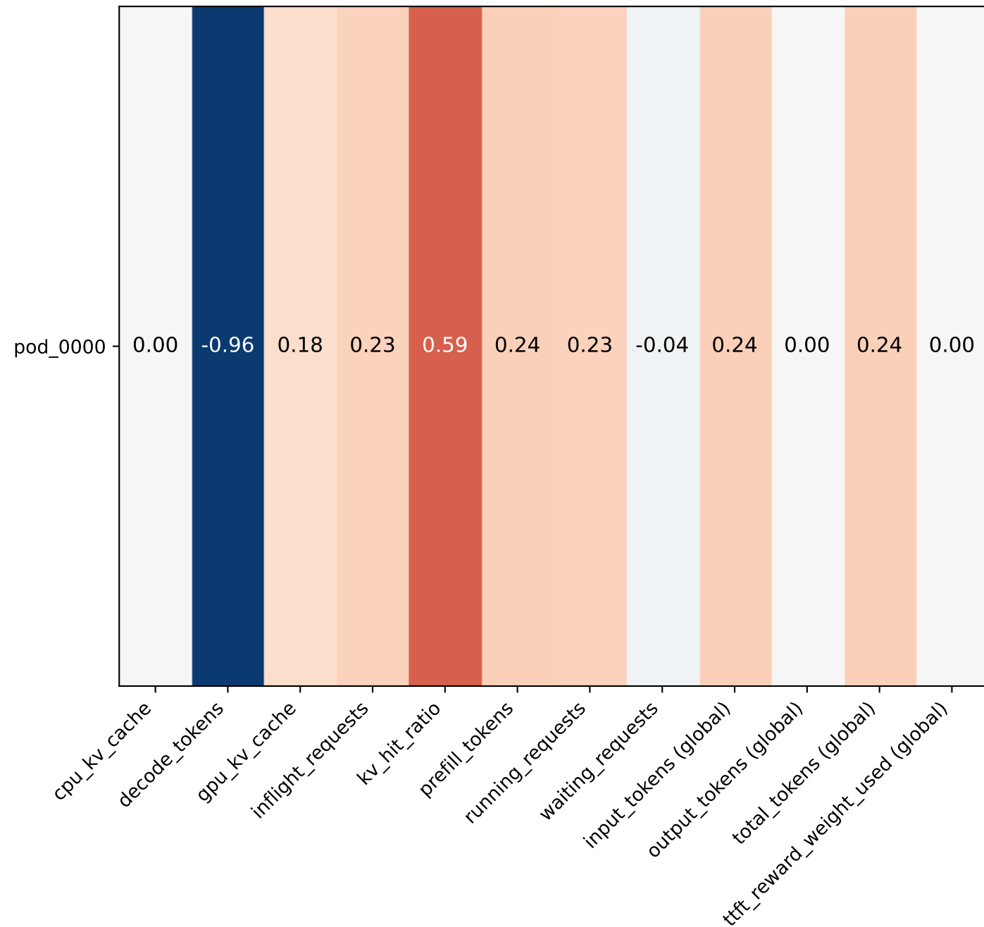
Pod State-Performance Correlations
