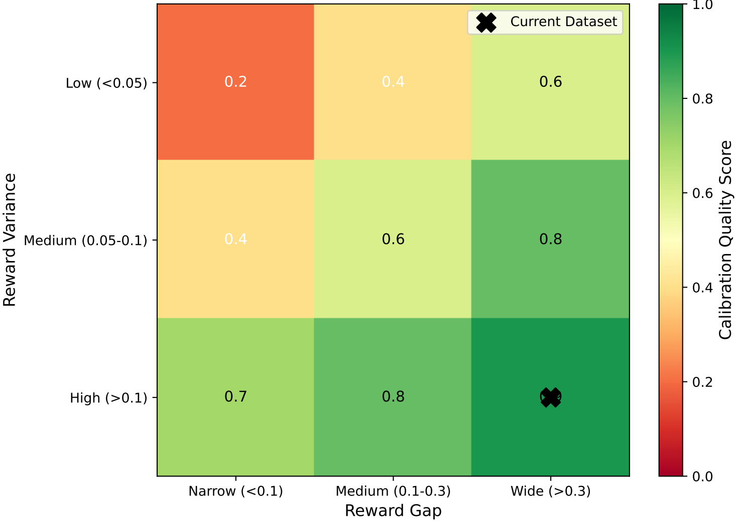
Confidence Calibration Prediction Matrix
