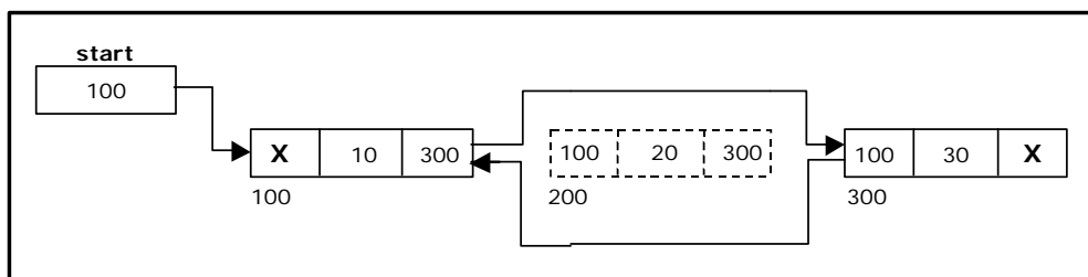
Figure 3.4.8 Deleting a node at an intermediate position
