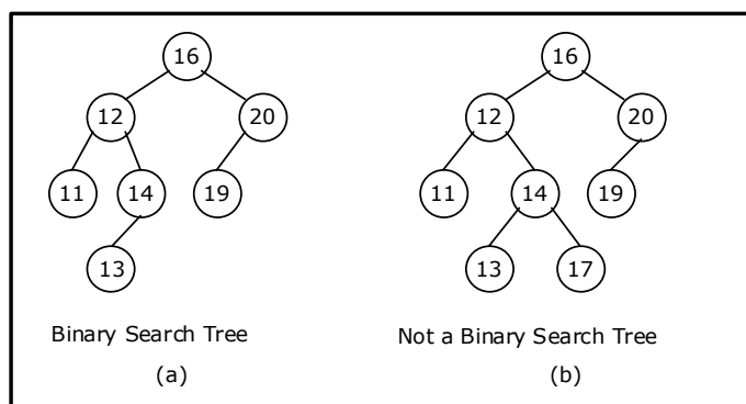
Figure 5.2.5. Examples of binary search trees
