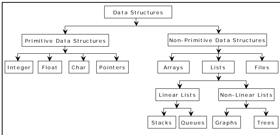
Figure 1.1. Classification of Data Structures
