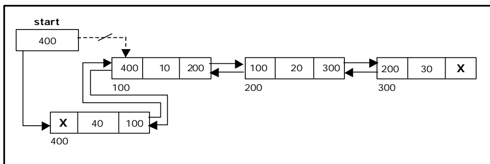
Figure 3.4.4. Inserting a node at the beginning
