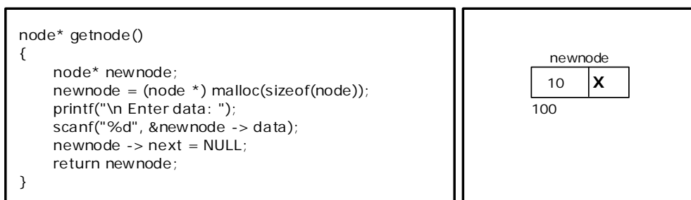
Figure 3.2.3. new node with a value of 10
