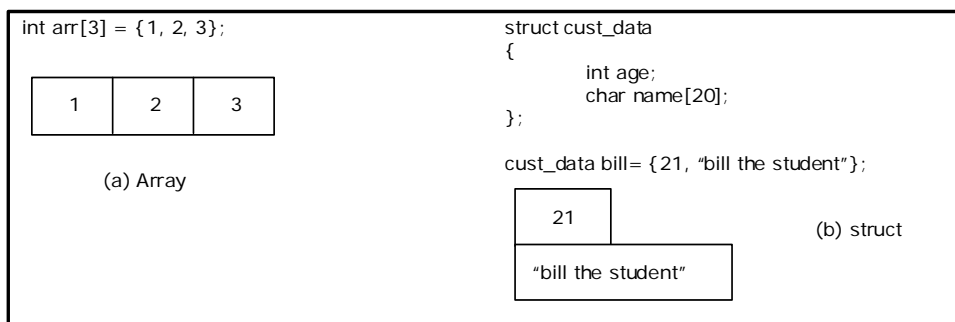
Figure 1.3 Examples of contiguous structures.
