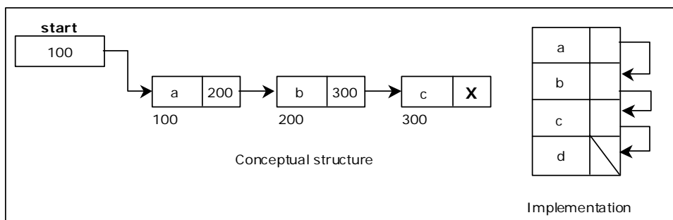
Figure 3.5.1. An array based linked list
