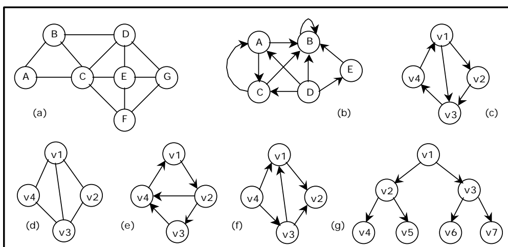
Figure 6.5.1 Various Graphs
