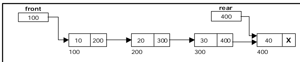
Figure 4.4. Linked Queue representation
