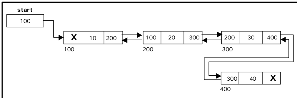
Figure 3.4.5. Inserting a node at the end
