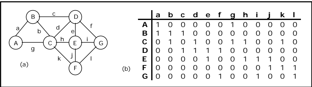
Figure 6.5.4 Graph and its incidence matrix
