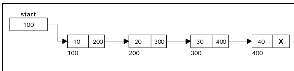
Figure 3.2.4. Single Linked List with 4 nodes
