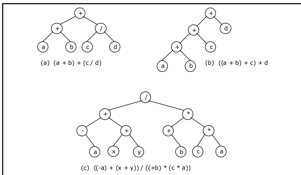
Figure 5.4.1 Expression Trees
