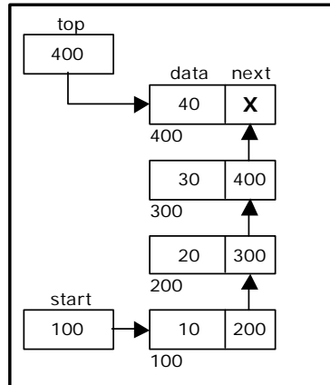
Figure 4.3. Linked stack representation
