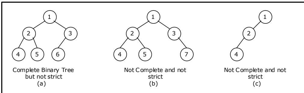
Figure 5.2.4. Examples of complete and incomplete binary trees
