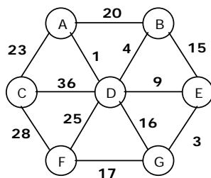
FIGURE 1 and its adjacency list
