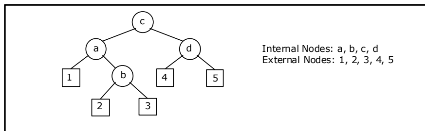
Figure 5.2.6. Internal and external nodes
