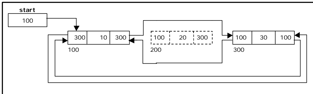
Figure 3.8.7. Deleting a node at an intermediate position
