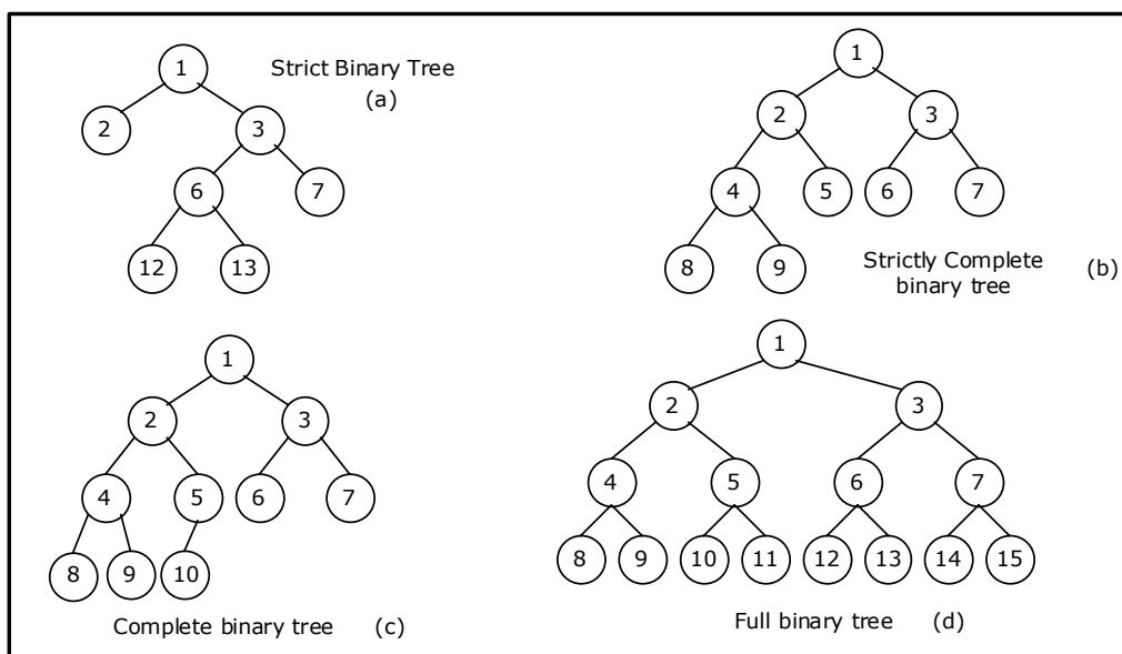
Figure 5.2.3. Examples of binary trees
