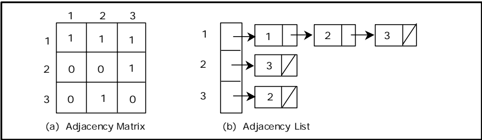
Figure 6.5.4 Adjacency matrix and adjacency list
