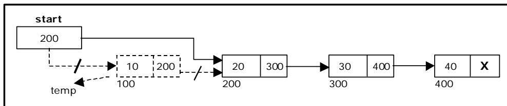
Figure 3.2.8. Deleting a node at the beginning.
