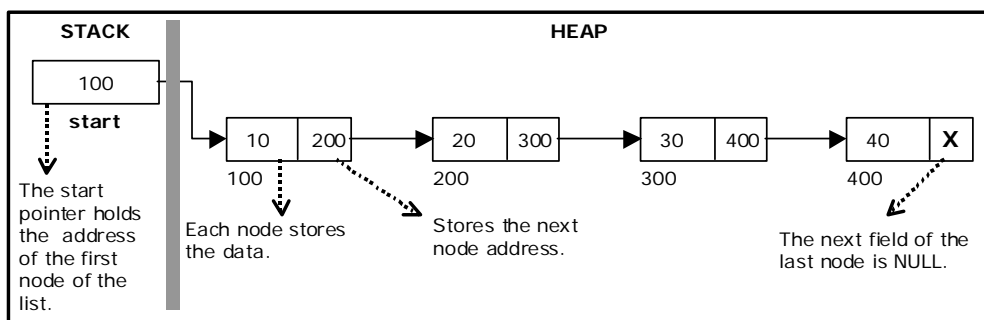
Figure 3.2.1. Single Linked List
