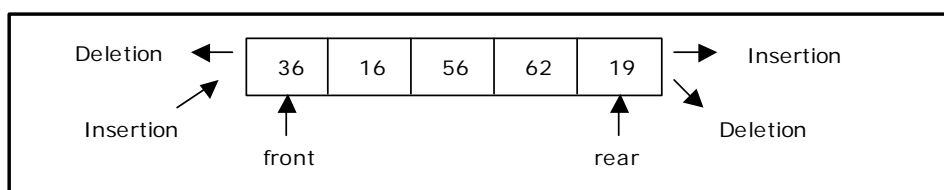
Figure 4.5. Representation of a deque.
