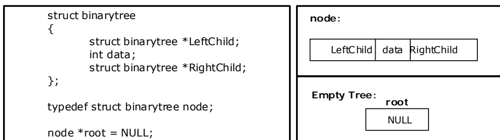
Figure 5.2.6. Structure definition, node representation and empty tree
