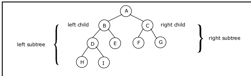
Figure 5.2.1. Binary Tree
