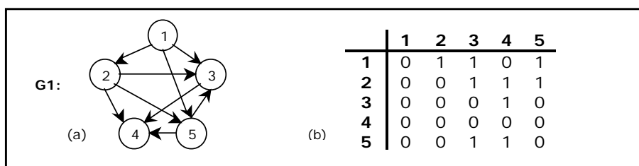
Figure 6.5.2. A graph and its Adjacency matrix
