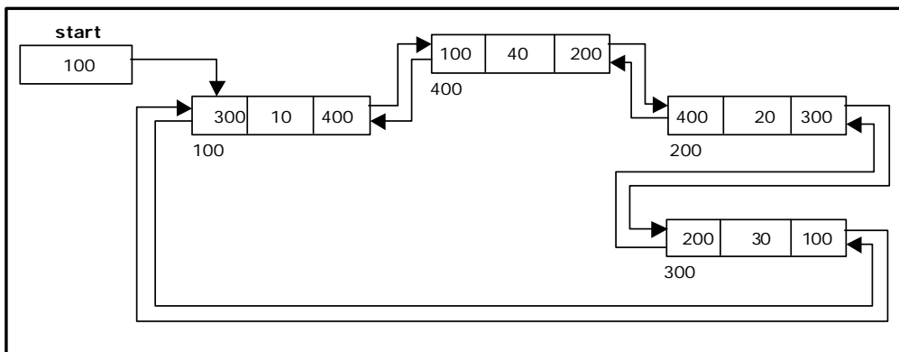
Figure 3.8.4. Inserting a node at an intermediate position
