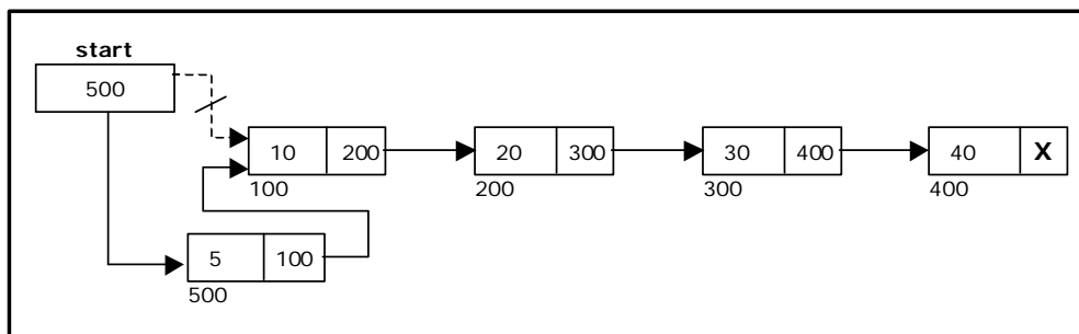
Figure 3.2.5. Inserting a node at the beginning
