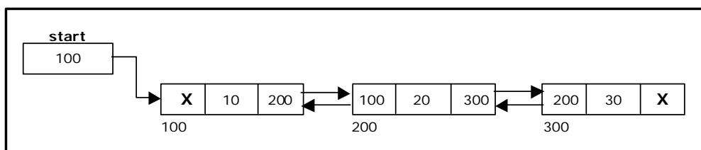
Figure 3.4.3. Double Linked List with 3 nodes
