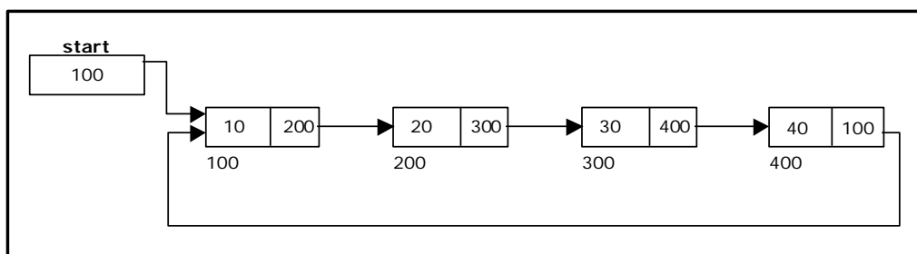
Figure 3.6.1. Circular Single Linked List
