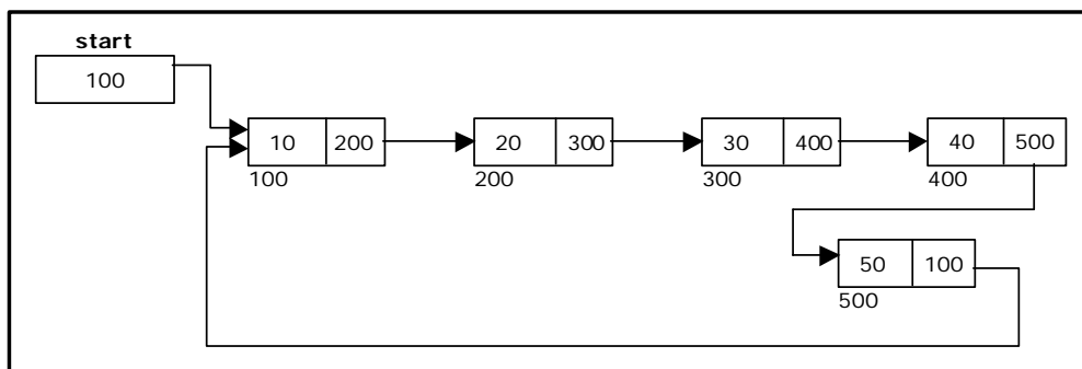
Figure 3.6.3 Inserting a node at the end.
