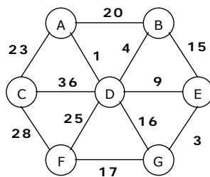
FIGURE 2 and its adjacency list
