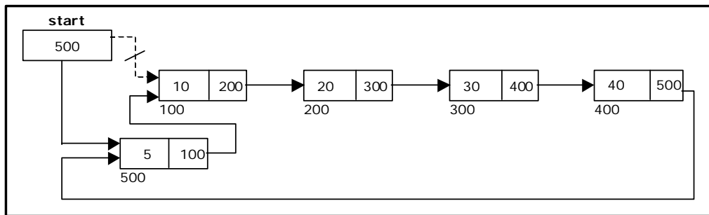
Figure 3.6.2. Inserting a node at the beginning
