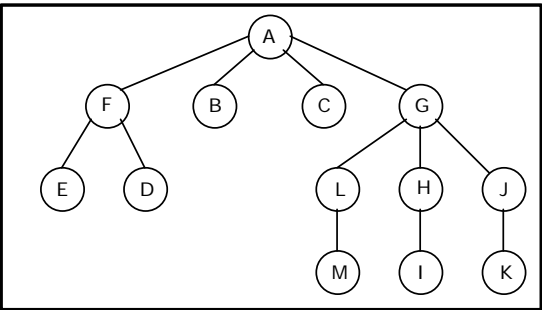
Breadth first traversal
