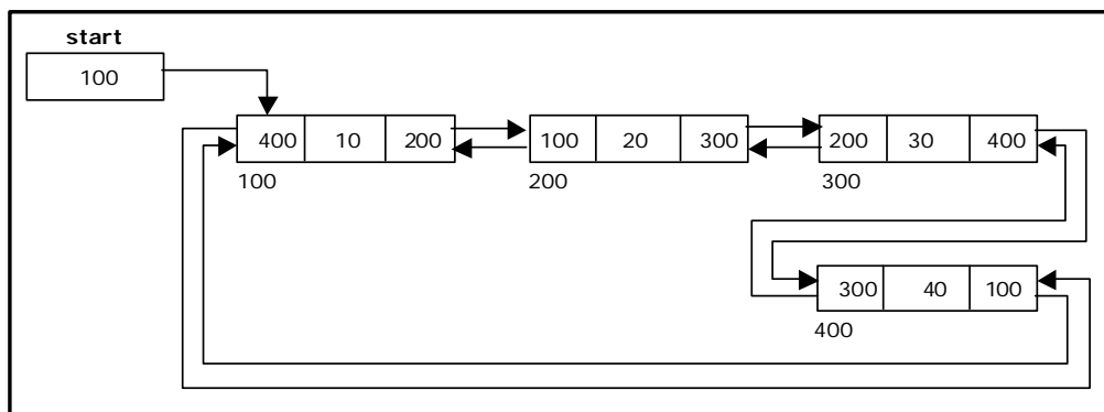
Figure 3.8.3. Inserting a node at the end
