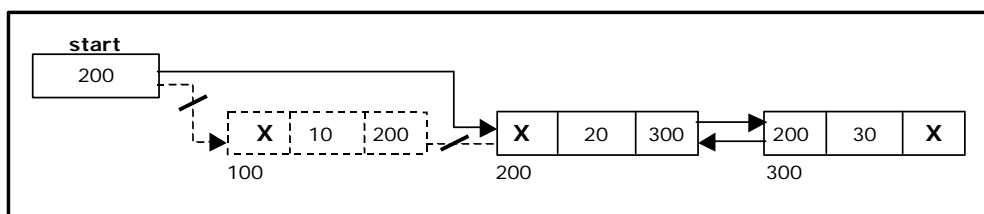
Figure 3.4.6. Deleting a node at beginning
