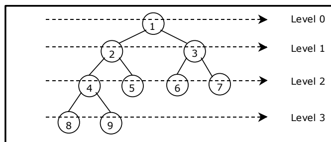
Figure 5.2.2. Level by level numbering of binary tree
