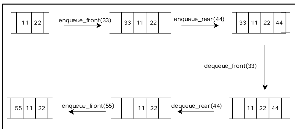
Figure 4.6. Basic operations on deque
