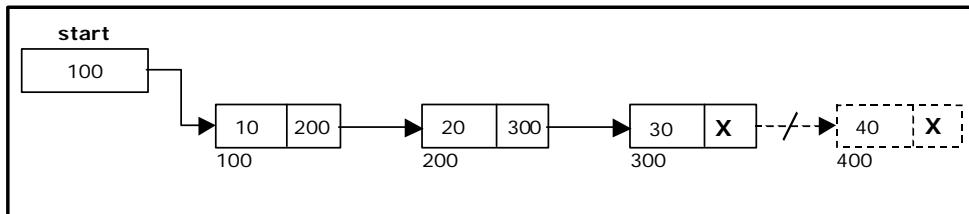
Figure 3.2.9. Deleting a node at the end.
