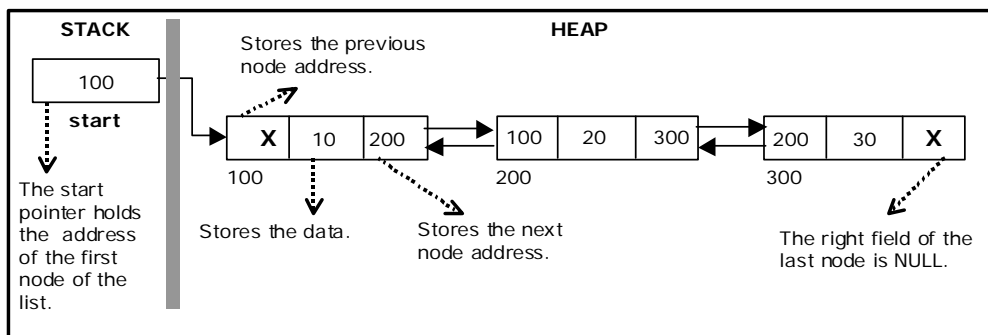
Figure 3.3.1. Double Linked List
