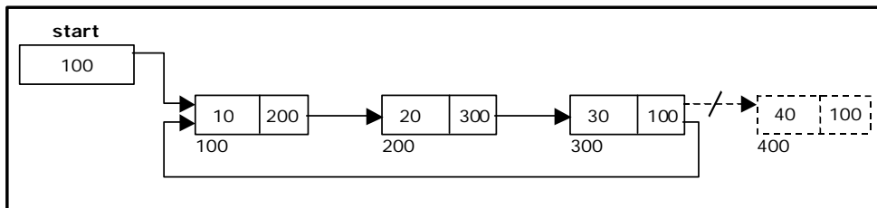
Figure 3.6.5. Deleting a node at the end.
