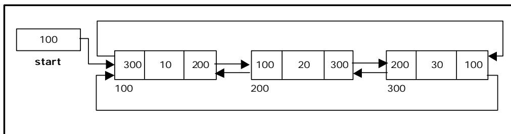
Figure 3.8.1. Circular Double Linked List
