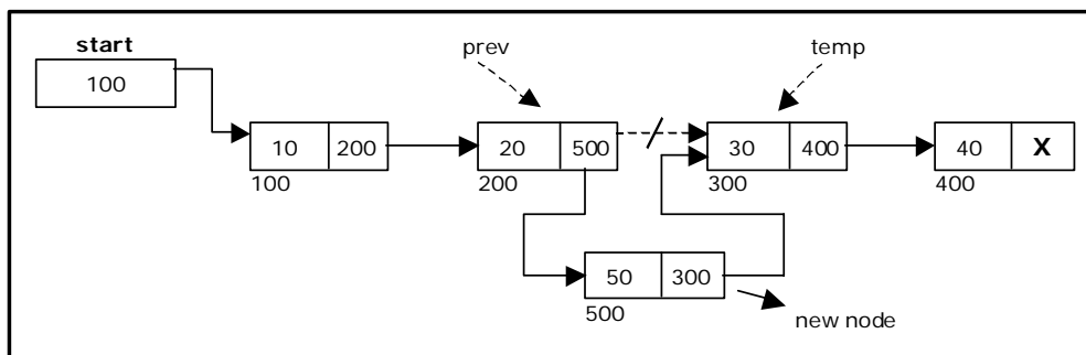
Figure 3.2.7. Inserting a node at an intermediate position.
