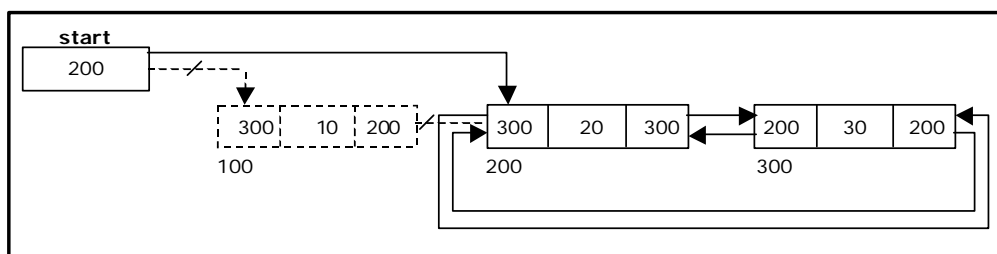
Figure 3.8.5. Deleting a node at beginning
