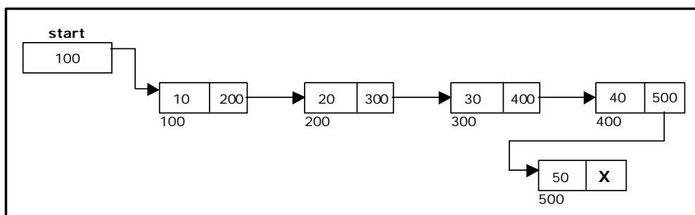
Figure 3.2.6. Inserting a node at the end.
