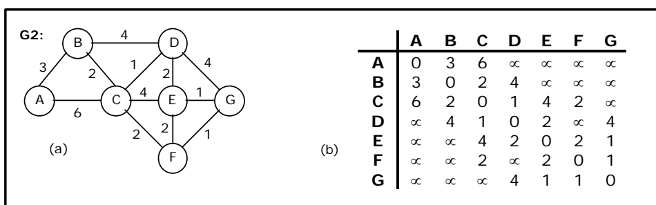
Figure 6.5.3 Weighted graph and its Cost adjacency matrix
