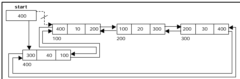
Figure 3.8.2. Inserting a node at the beginning
