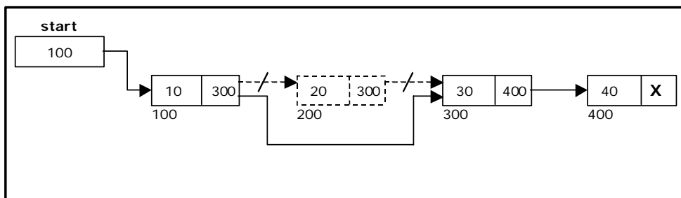
Figure 3.2.10. Deleting a node at an intermediate position.
