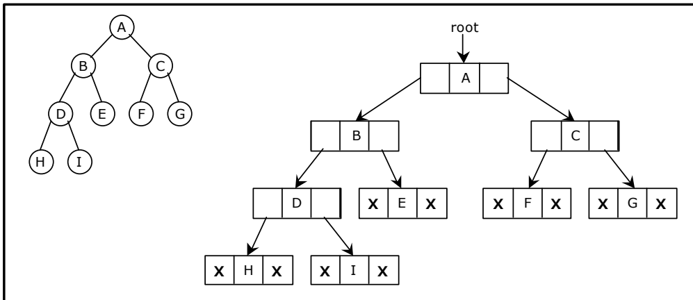
Figure 5.2.7. Linked representation for the binary tree
