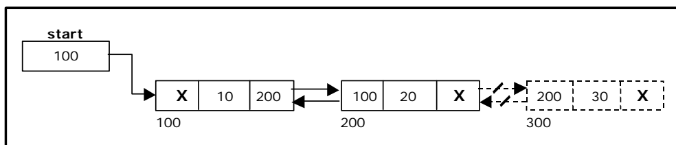
Figure 3.4.7. Deleting a node at the end
