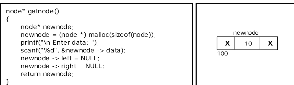
Figure 3.4.2. new node with a value of 10
