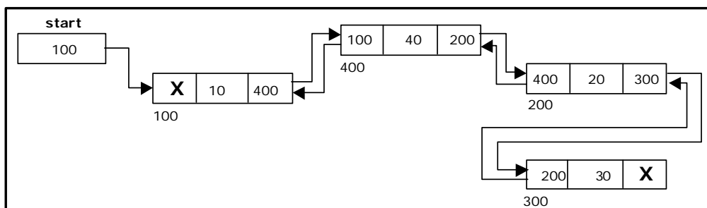
Figure 3.4.6. Inserting a node at an intermediate position
