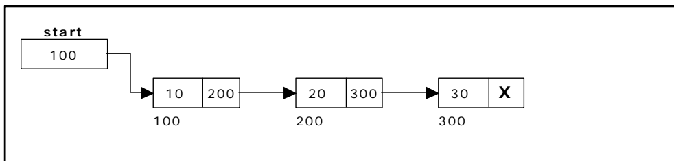
Single Linked List without a header node
