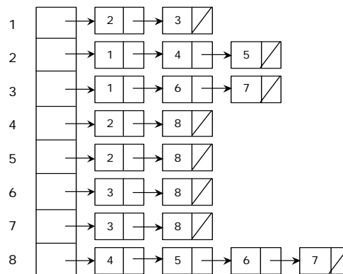
Adjacency list for graph G
