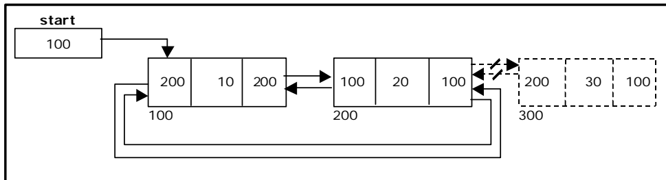
Figure 3.8.6. Deleting a node at the end
