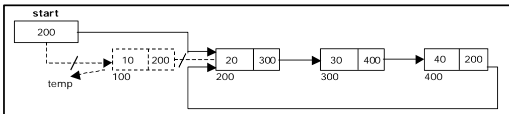
Figure 3.6.4. Deleting a node at beginning.
