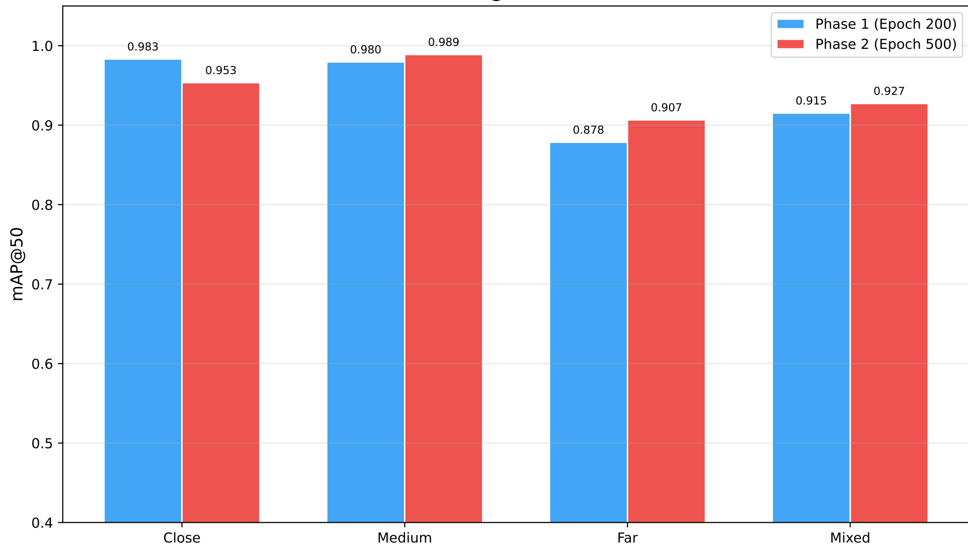
Distance-Wise mAP@50: Phase 1 vs Phase 2
