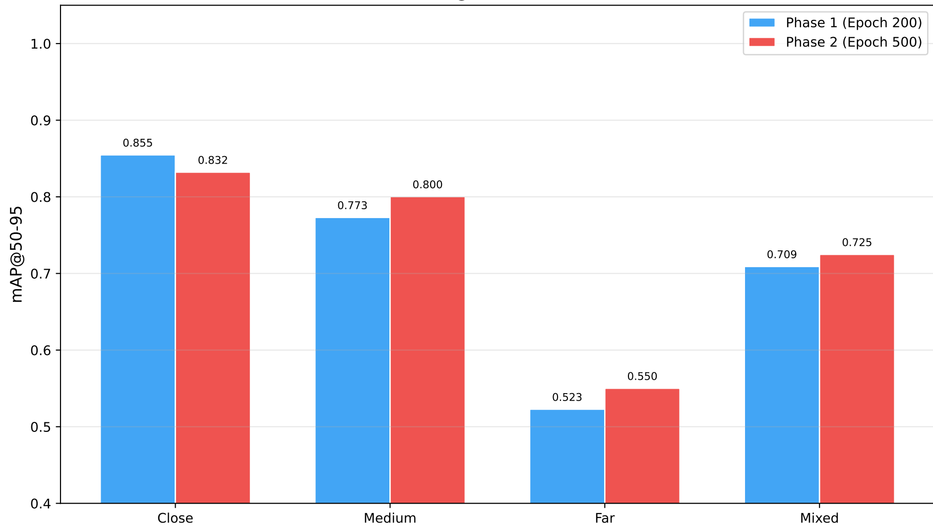
Distance-Wise mAP@50-95: Phase 1 vs Phase 2
