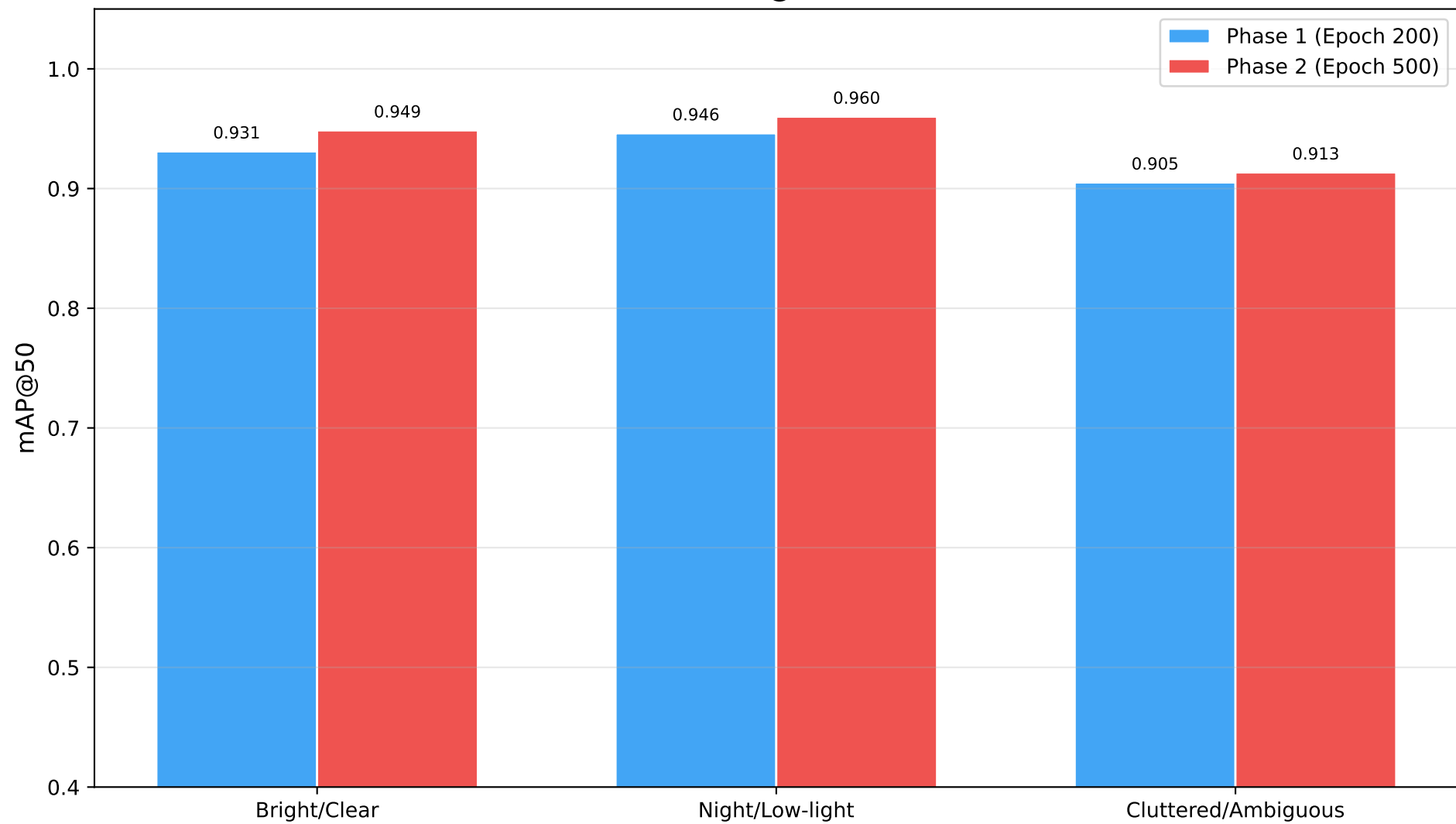
Environment-Wise mAP@50: Phase 1 vs Phase 2
