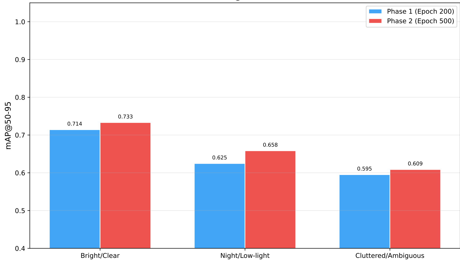
Environment-Wise mAP@50-95: Phase 1 vs Phase 2
