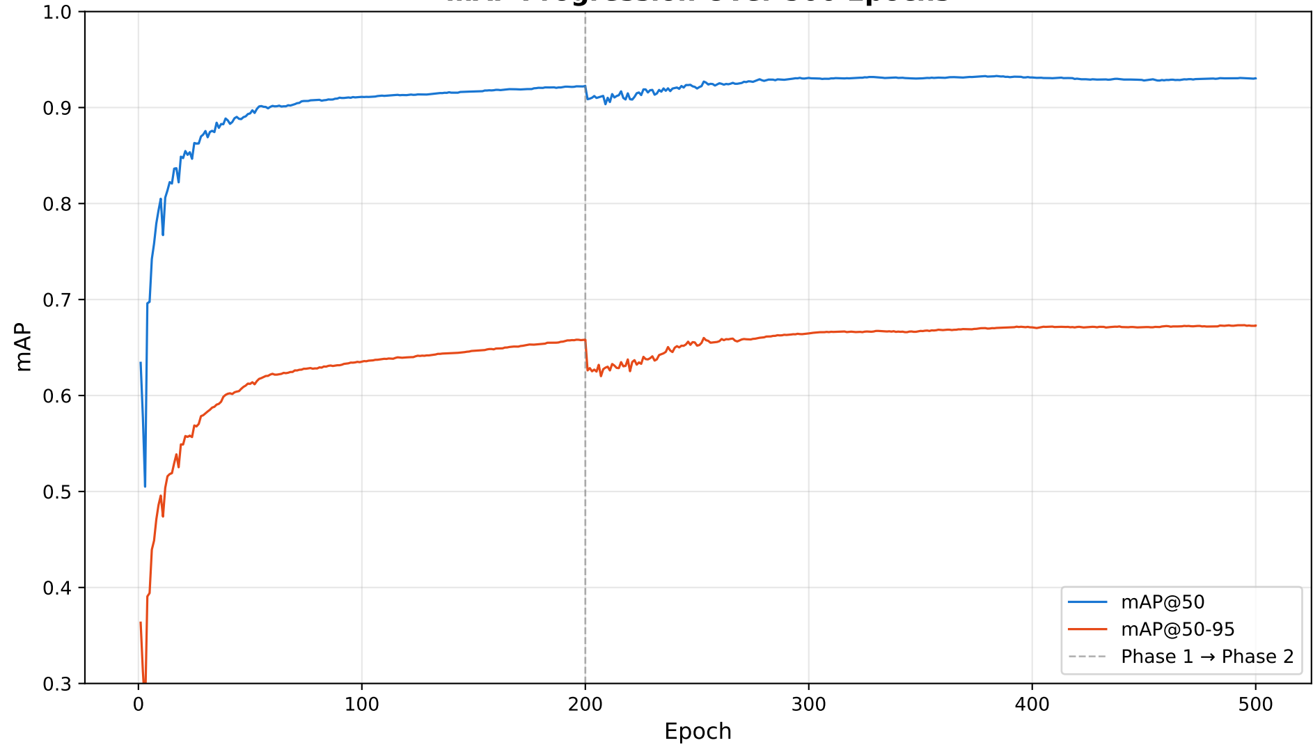
mAP Progression Over 500 Epochs
