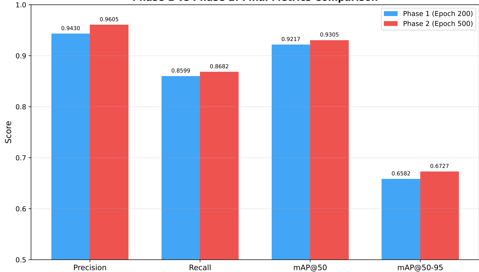
Phase 1 vs Phase 2: Final Metrics Comparison
