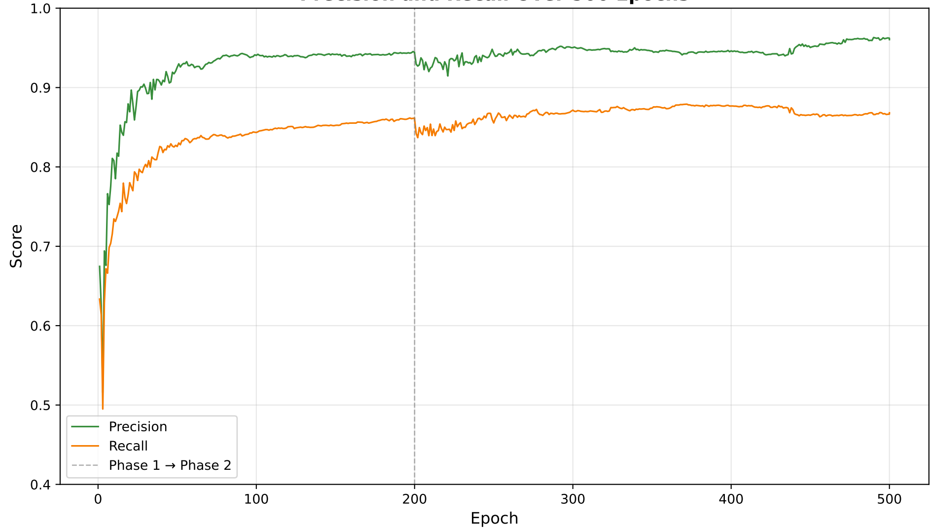
Precision and Recall Over 500 Epochs
