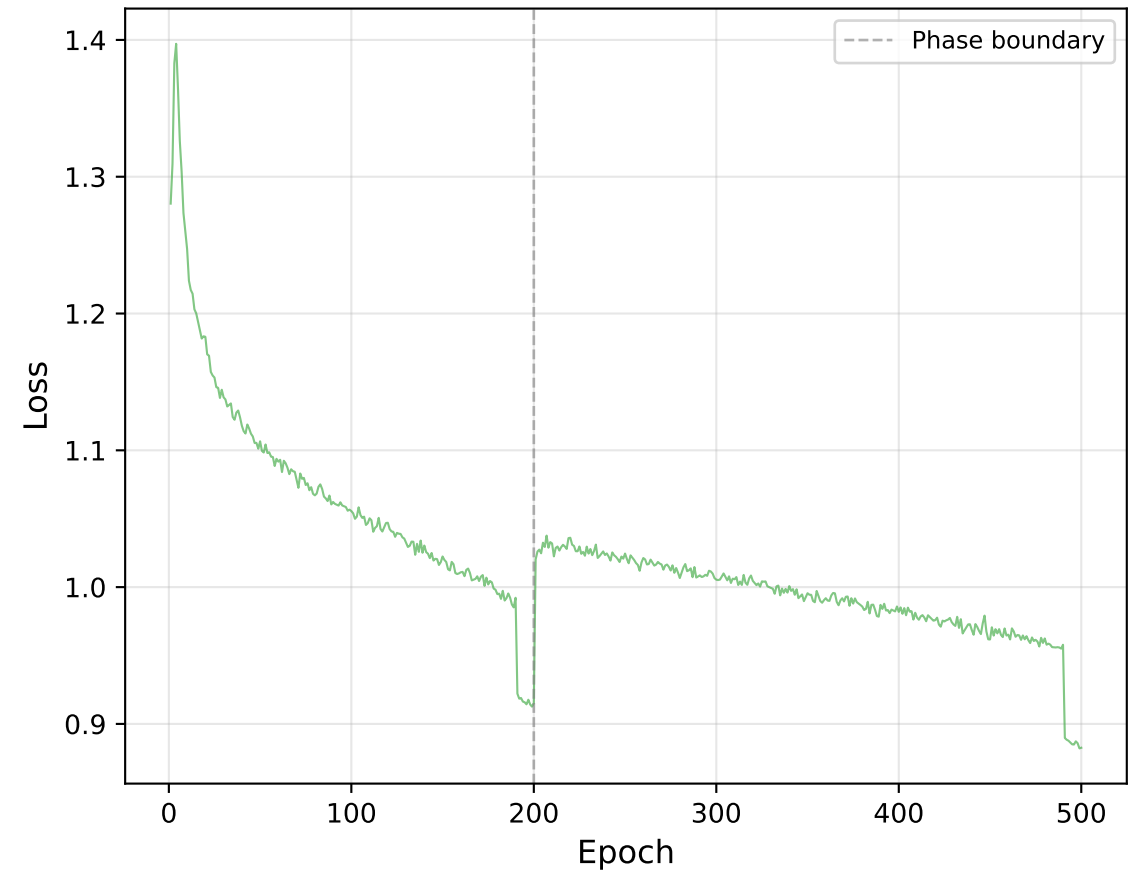
DFL Loss
