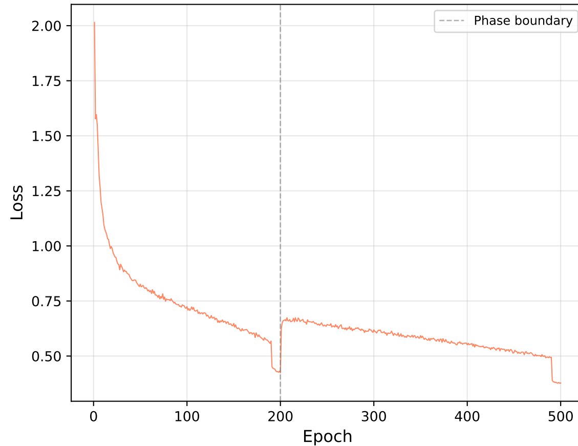
Classification Loss
