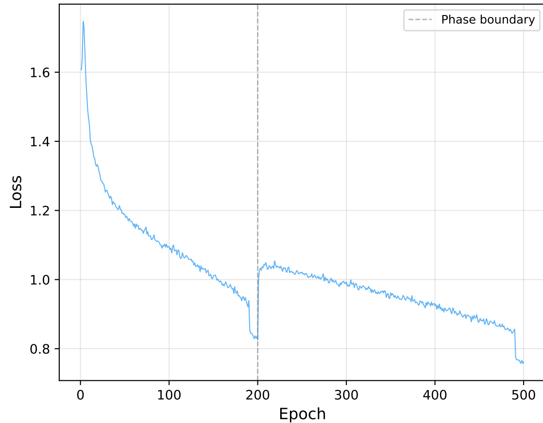
Box Loss
