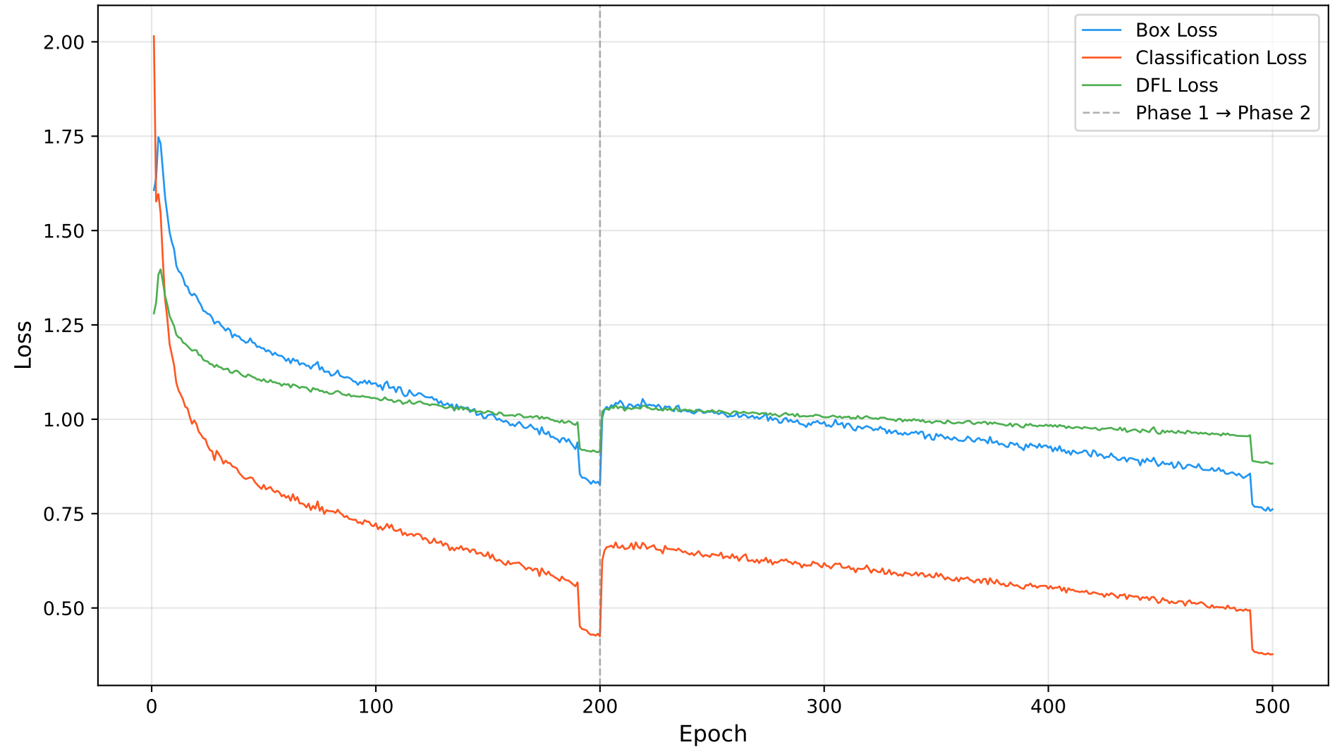
Training Losses Over 500 Epochs
