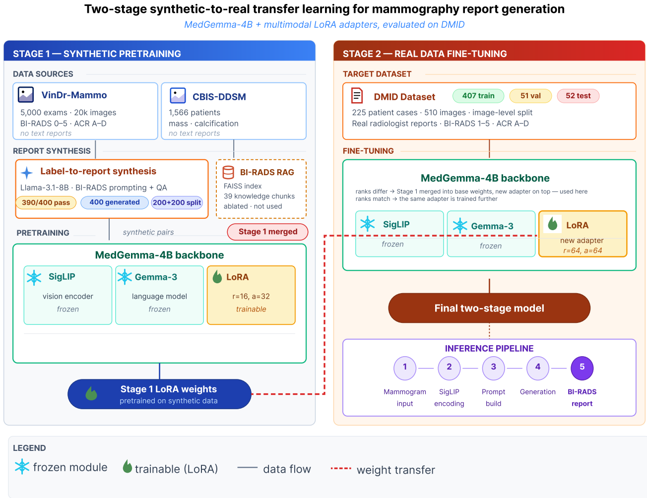
Figure 1. Overview of the two-stage synthetic-to-real transfer learning framework. Stage 1 pretrains on synthetic reports generated from structured BI-RADS annotations in VinDr-Mammo and CBIS-DDSM: 400 reports are generated and 390 pass automated validation (97.5%). Stage 2 transfers the pretrained LoRA weights and fine-tunes on real radiologist reports from DMID. Two transfer mechanisms exist—continued training of the same adapter when the Stage 1 and Stage 2 ranks match, or merging Stage 1 into the base weights (Eq. 7) and training a new adapter when they do not. The BI-RADS retrieval module is shown as ablated and is not part of the inference path: the retrieval ablation shows that it degrades generation, and it is reported as a negative result.
