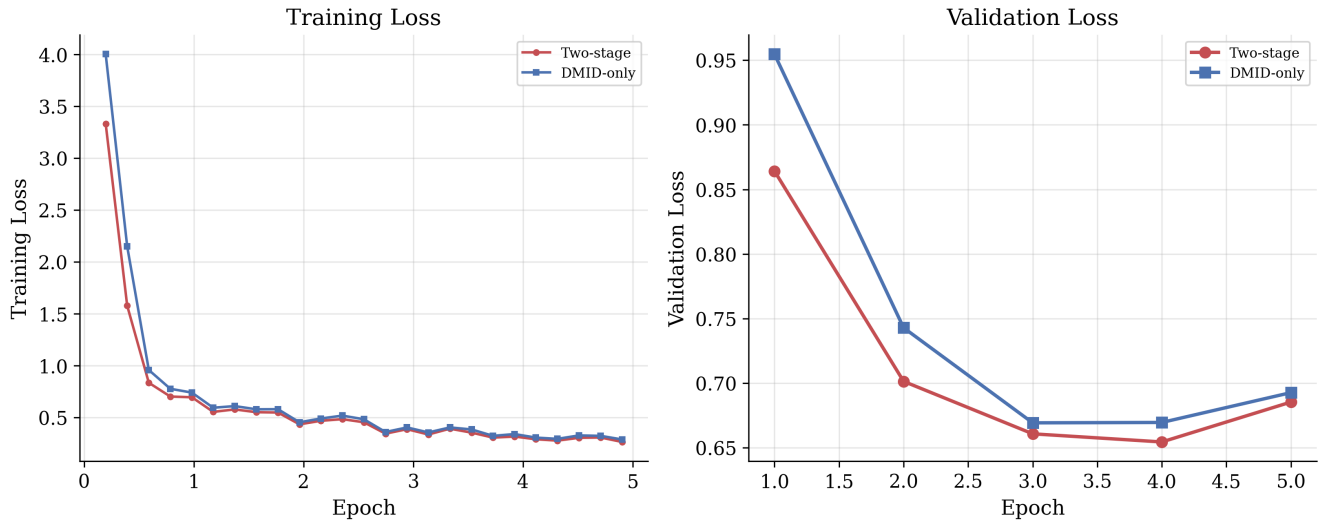
Figure 4. Training dynamics. Two-stage benefits from lower initial loss and achieves lower best validation loss (0.655 vs. 0.669).
