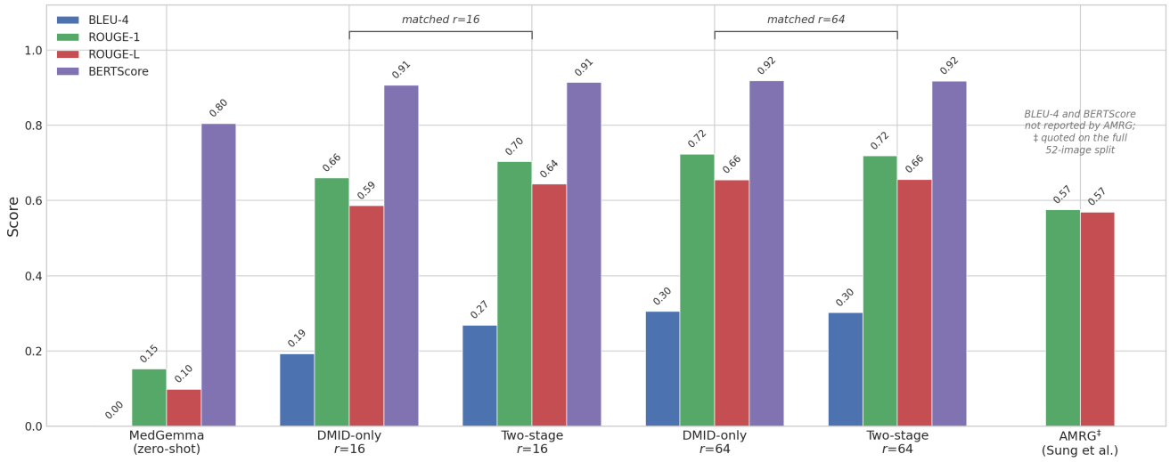
Figure 2. DMID test set comparison across key methods on the leak-free subset ( n = 49 ), with the two training schemes shown at matched adapter rank. The AMRG bars are quoted on the full 52-image split as published and are marked accordingly. At r = 64 the two schemes are visually indistinguishable on every metric.
