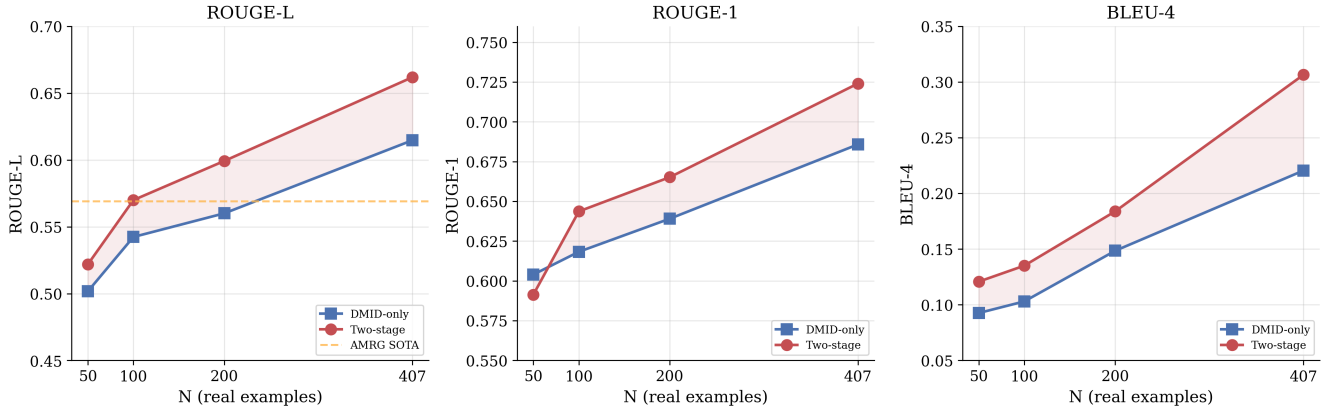
Figure 3. Data efficiency analysis under the protocol of Supplementary Table S2 ( r = 16 , one initialisation per point). Error bars are unavailable because per-sample generations were not retained; the separation between the curves is smaller than the between-initialisation variability measured for a fixed configuration elsewhere in this study, and no data-efficiency claim is drawn from it.
