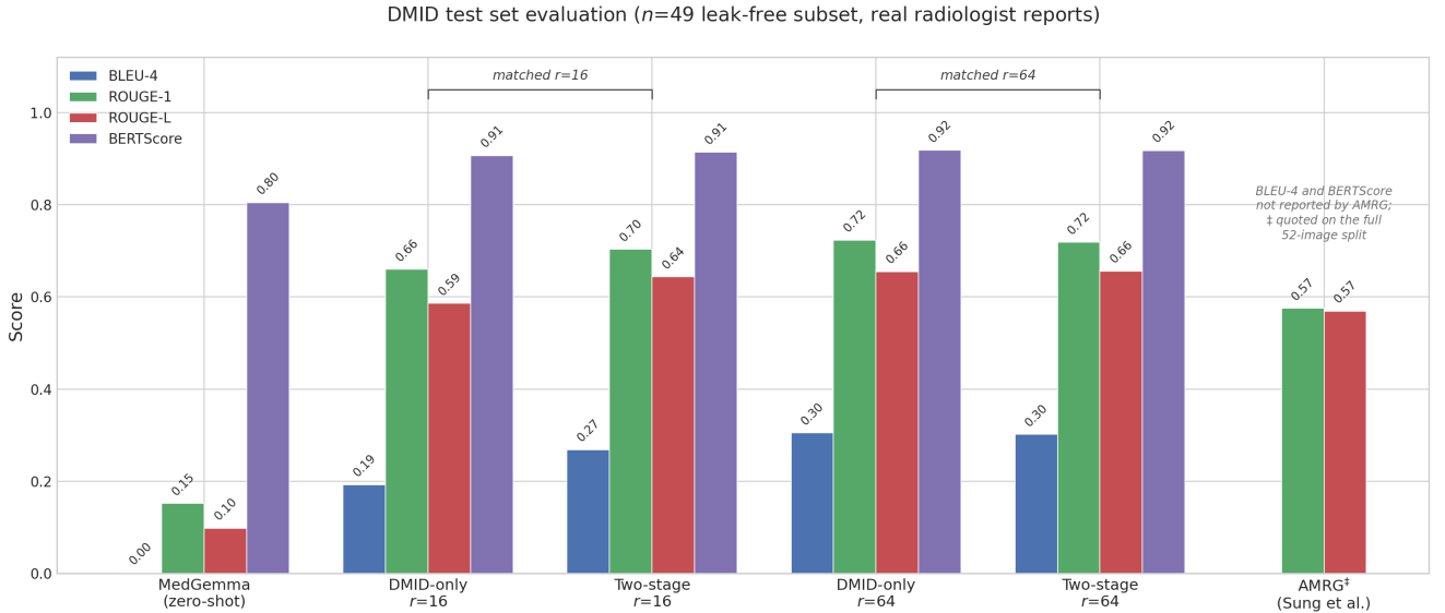
Figure 2. DMID test set comparison across key methods on the leak-free subset ( n = 49 ) , with the two training schemes shown at matched adapter rank. The AMRG bars are quoted on the full 52-image split as published and are marked accordingly. At r = 64 the two schemes are visually indistinguishable on every metric.
