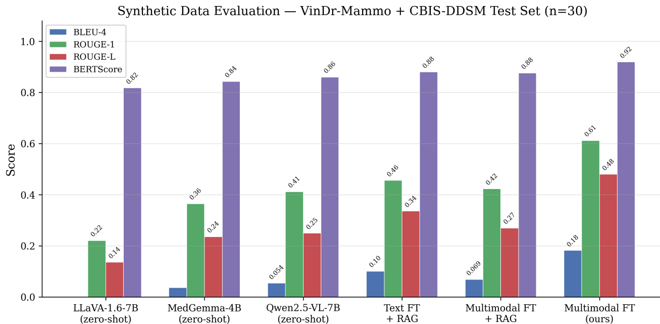
Figure S1: Stage 1 evaluation on synthetic test data. Multimodal fine-tuning without RAG achieves the best NLP metrics across all measures.
