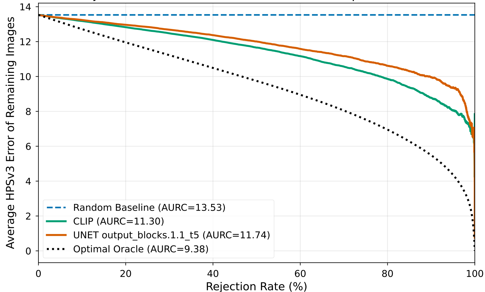
Rejection Curve: CLIP vs Internal UNET vs Optimal Bound
