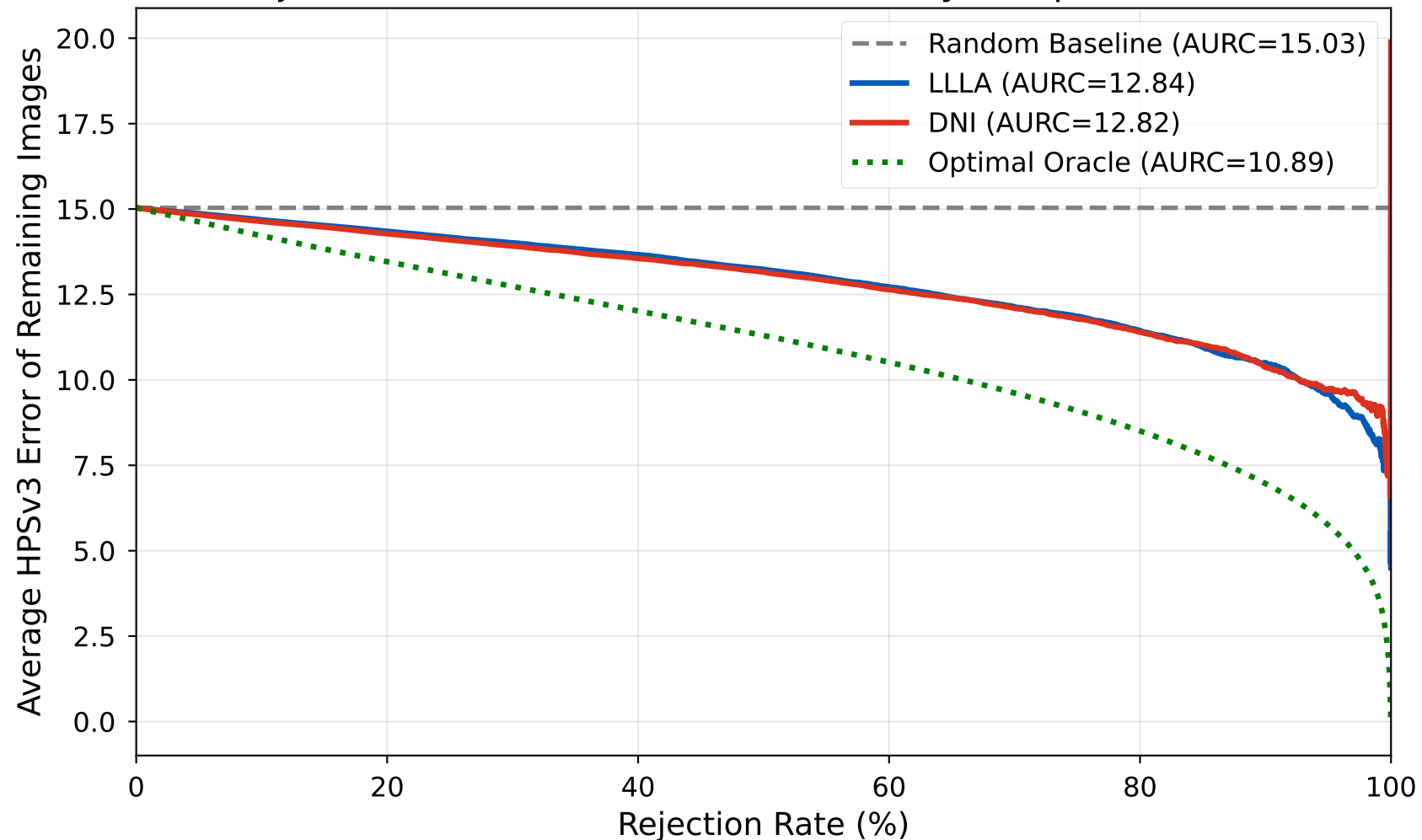
Rejection Curve: Generative Uncertainty vs Optimal Bound
