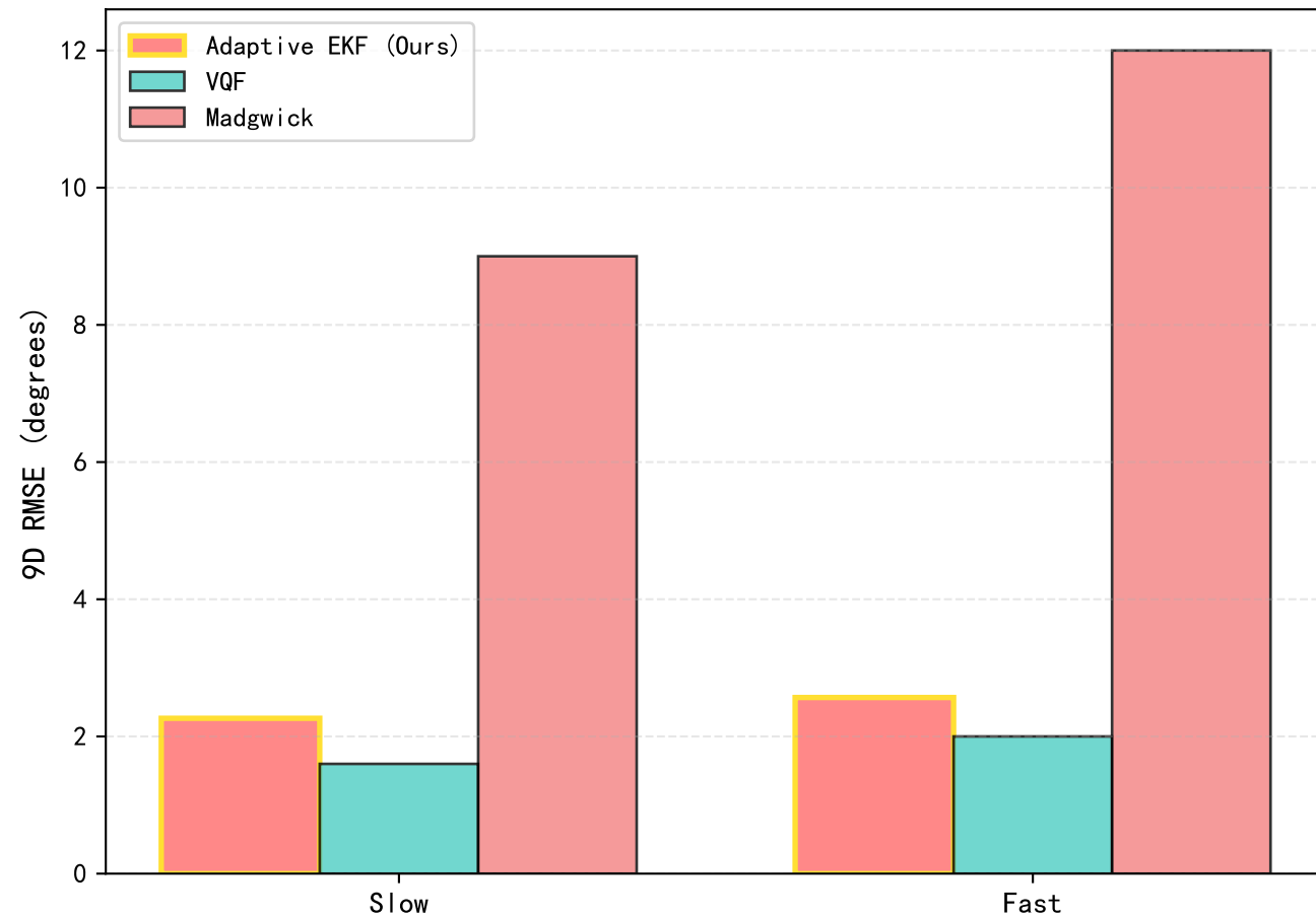
Motion Speed Comparison (Inertial Frame Filtering)
