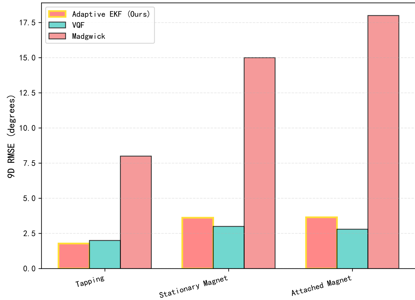
Magnetic Disturbance Comparison (Dip Angle Gating)
