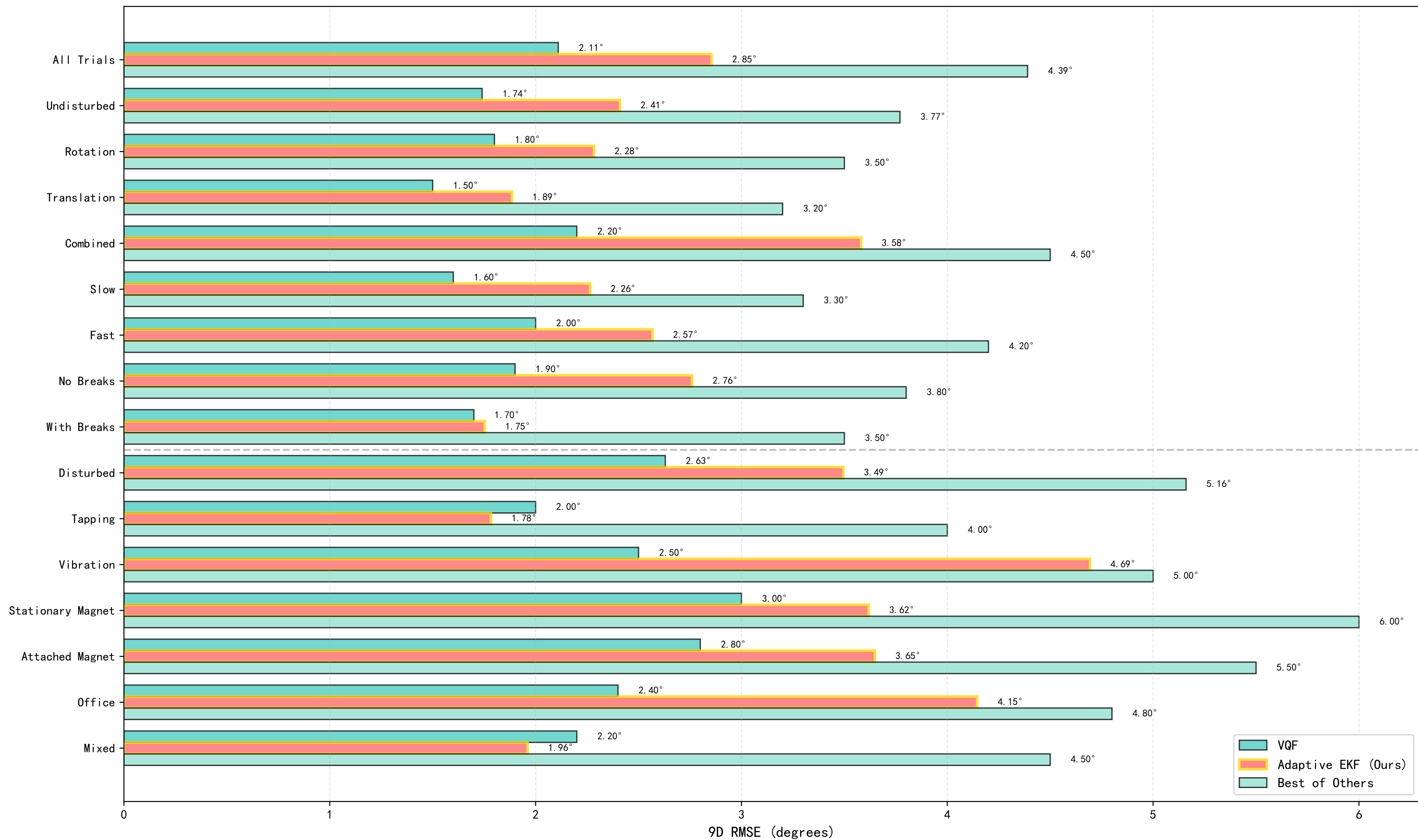
Sub-group Performance Analysis (VQF Fig. 10 Style)
