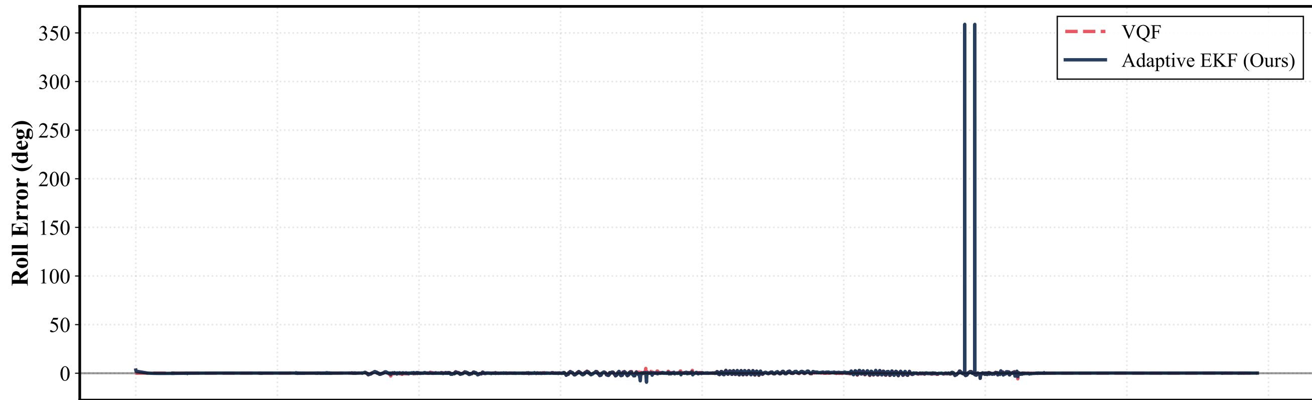
Euler Angle Error Comparison - 06_undisturbed_fast_rotation_A
