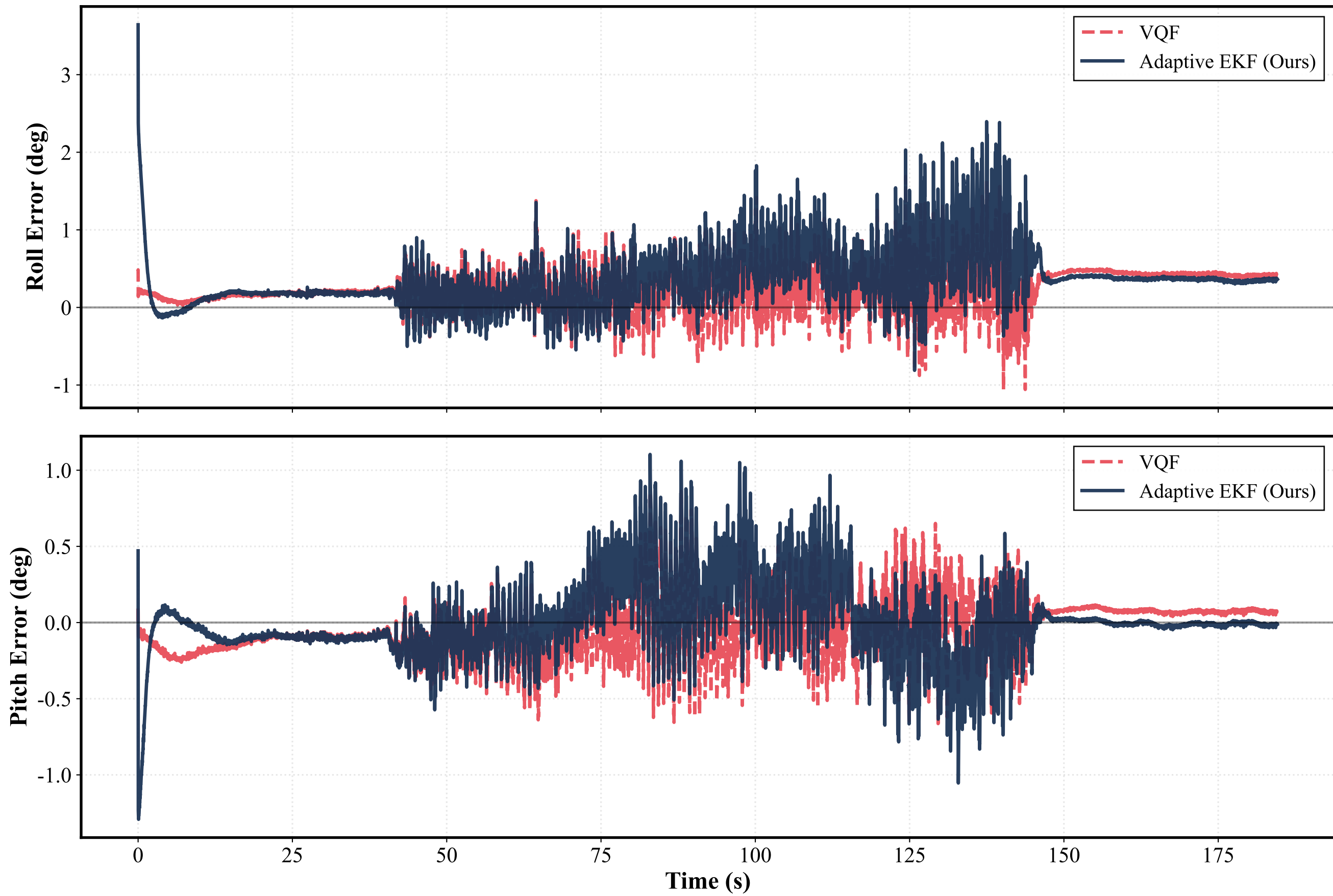
Euler Angle Error Comparison - 15_undisturbed_fast_translation_A
