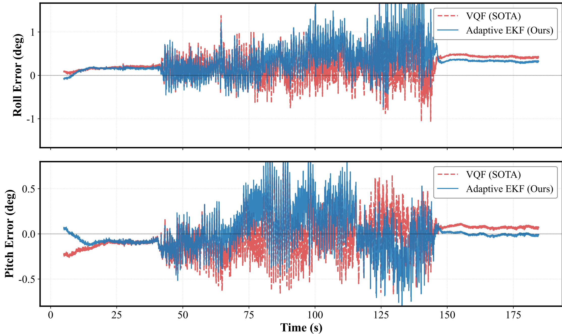
Euler Angle Error Comparison - 15_undisturbed_fast_translation_A (Initialization phase excluded)
