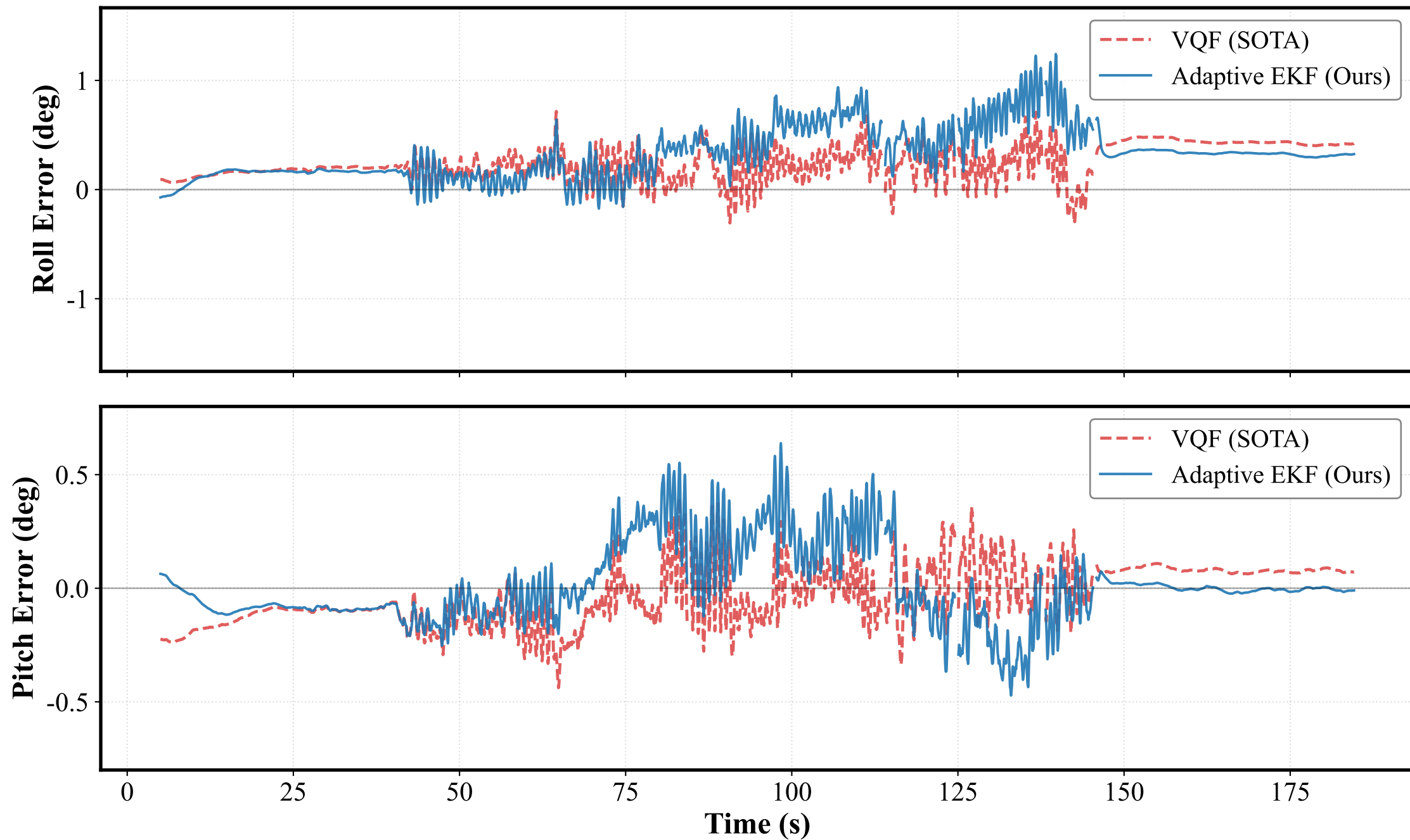
Euler Angle Error Comparison - 15_undisturbed_fast_translation_A (Initialization phase excluded (Smoothed: 0.5s window))
