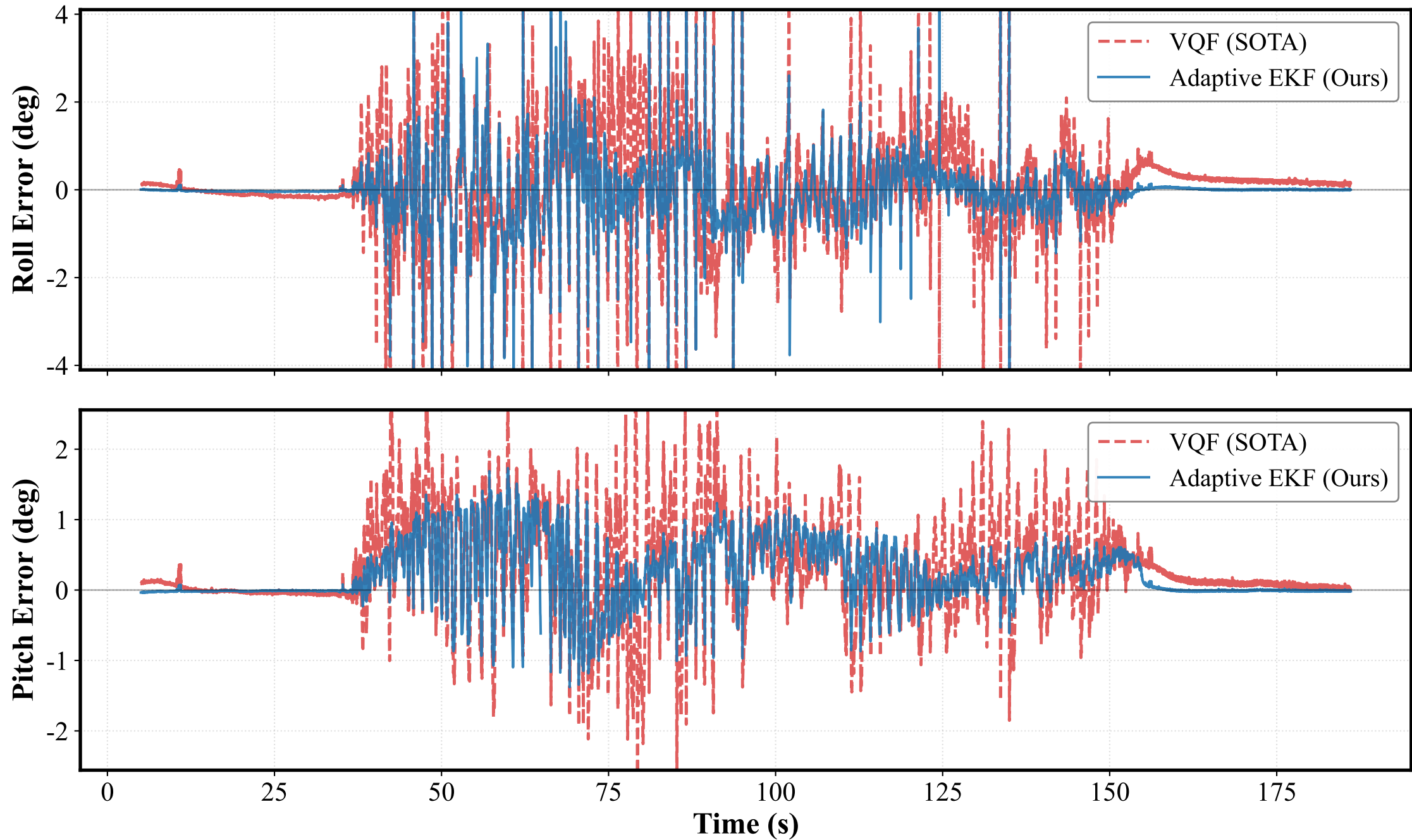
Euler Angle Error Comparison - 21_undisturbed_fast_combined (Initialization phase excluded)
