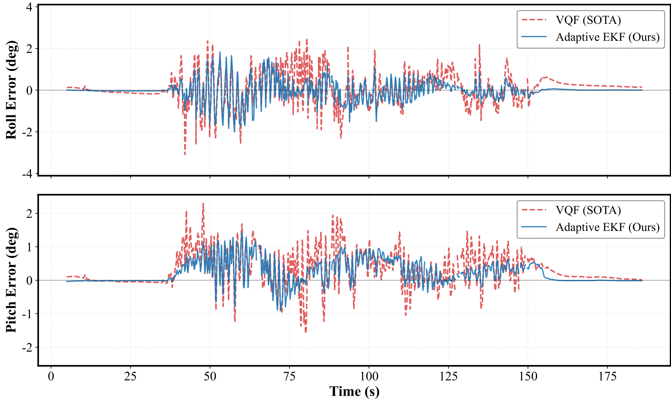
Euler Angle Error Comparison - 21_undisturbed_fast_combined (Initialization phase excluded (Smoothed: 0.5s window))
