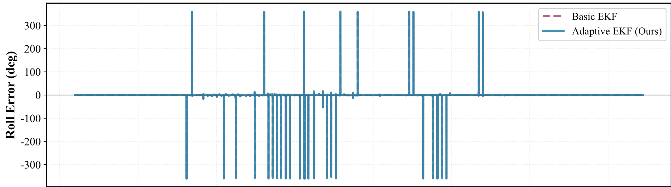
Euler Angle Error Comparison - 21_undisturbed_fast_combined
