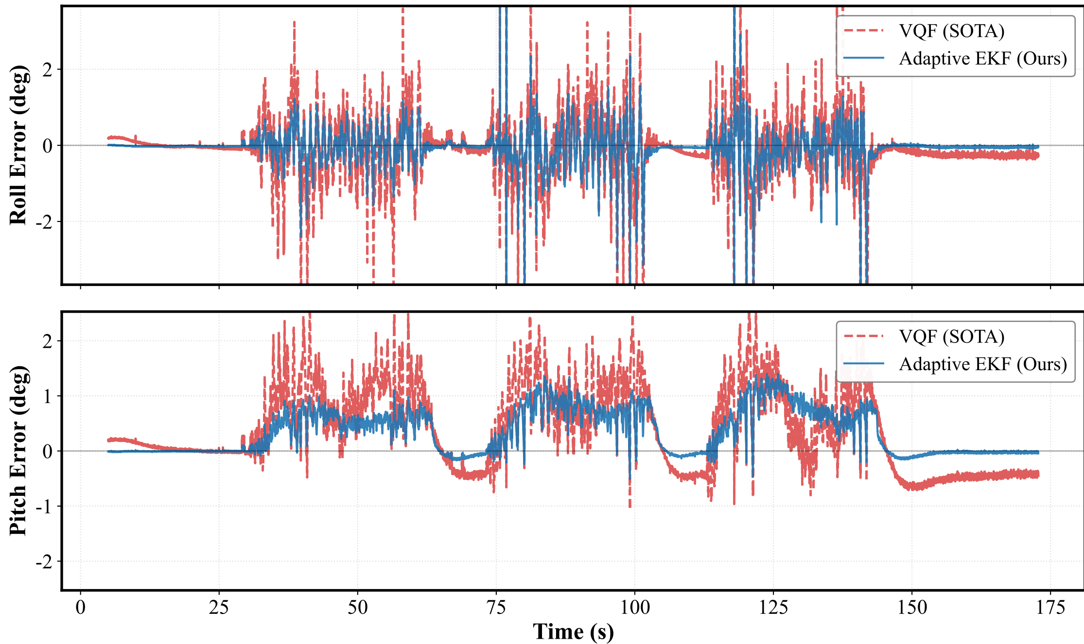
Euler Angle Error Comparison - 30_disturbed_stationary_magnet_C (Initialization phase excluded)
