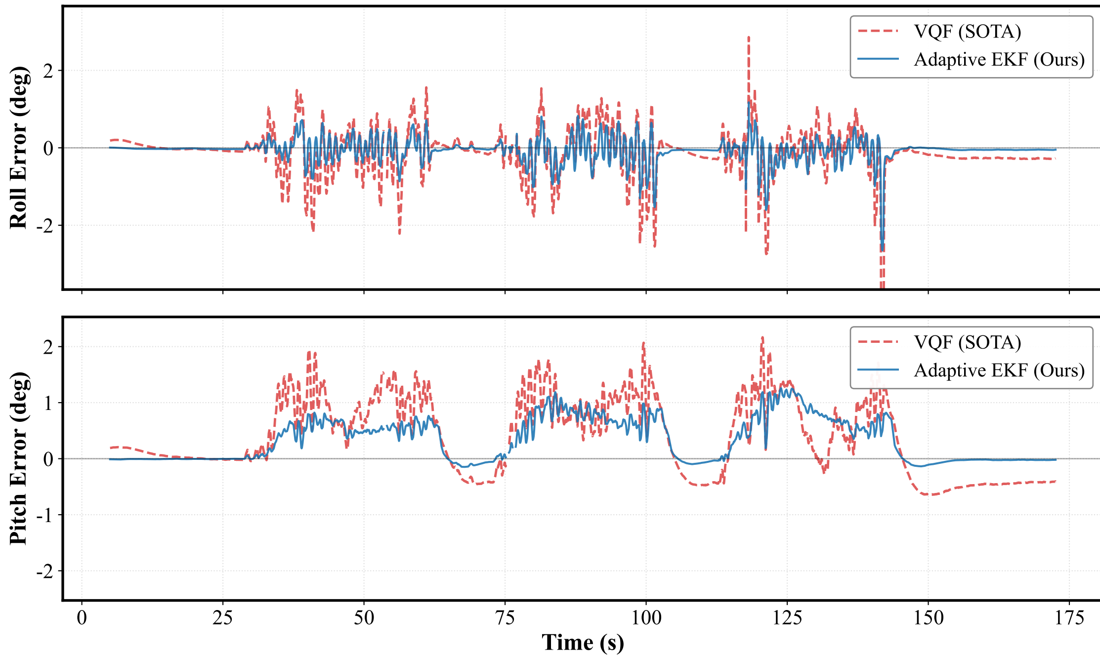
Euler Angle Error Comparison - 30_disturbed_stationary_magnet_C (Initialization phase excluded (Smoothed: 0.5s window))
