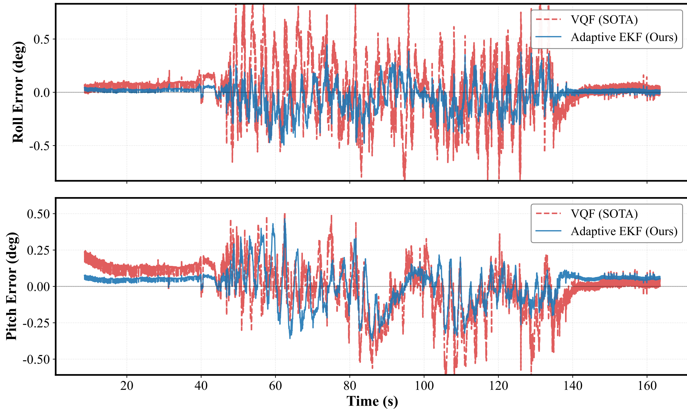
Euler Angle Error Comparison - 33_disturbed_attached_magnet_2cm (Initialization phase excluded)
