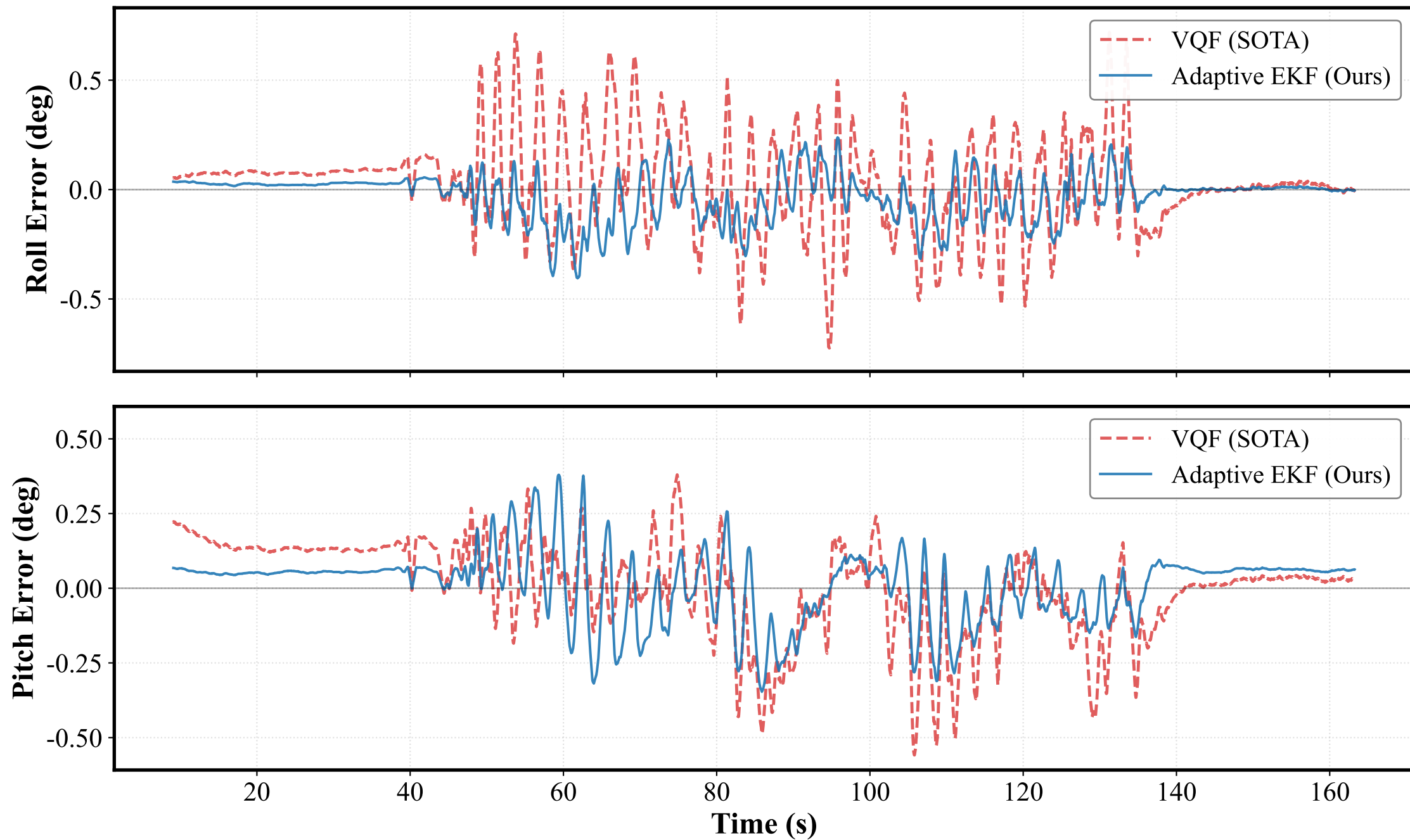
Euler Angle Error Comparison - 33_disturbed_attached_magnet_2cm (Initialization phase excluded (Smoothed: 0.5s window))
