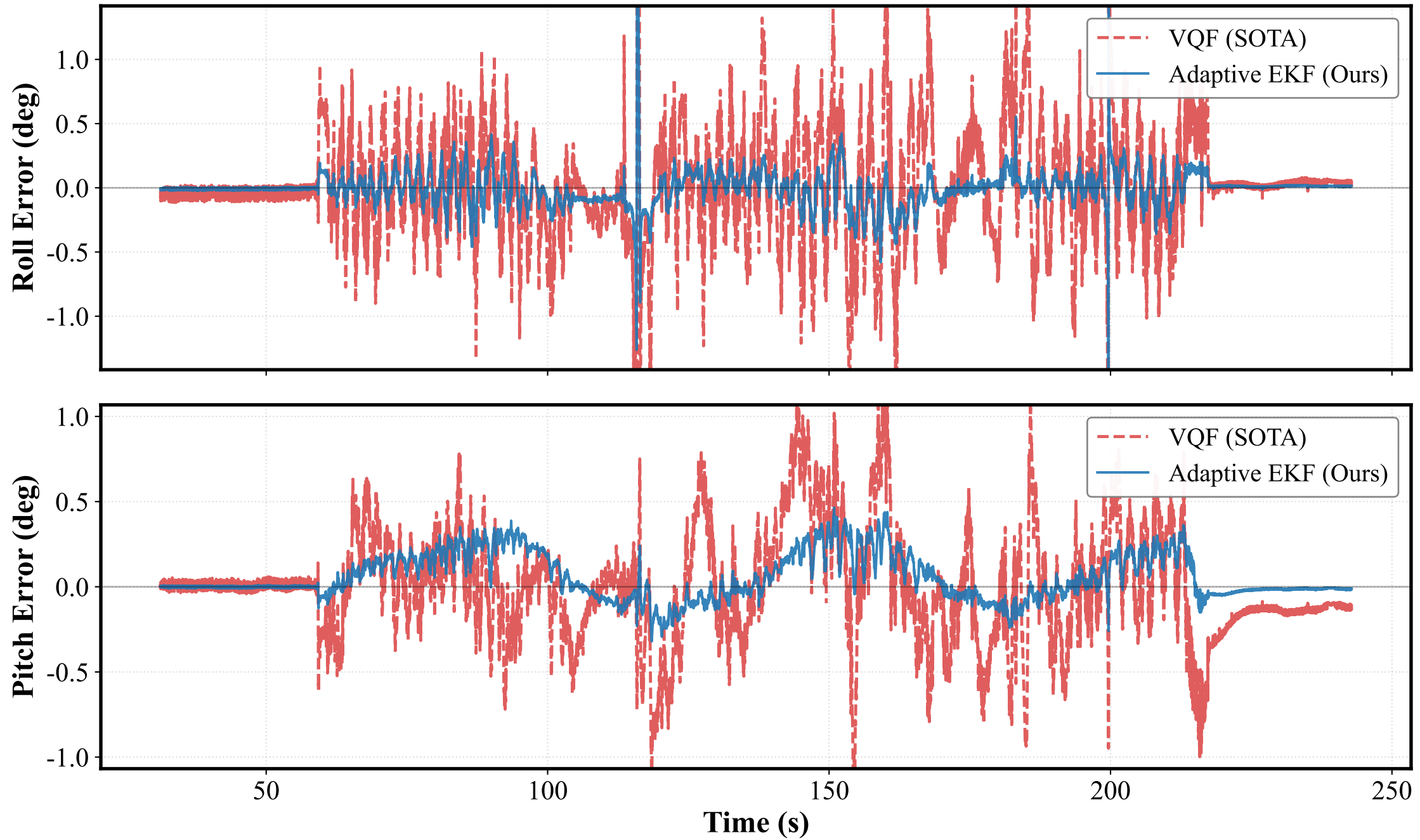
Euler Angle Error Comparison - 37_disturbed_office_A (Initialization phase excluded)
