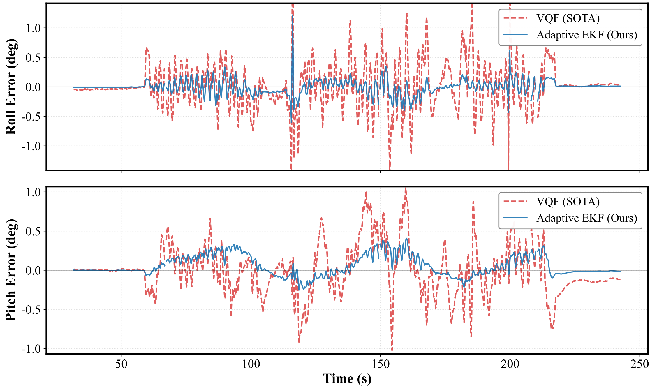
Euler Angle Error Comparison - 37_disturbed_office_A (Initialization phase excluded (Smoothed: 0.5s window))
