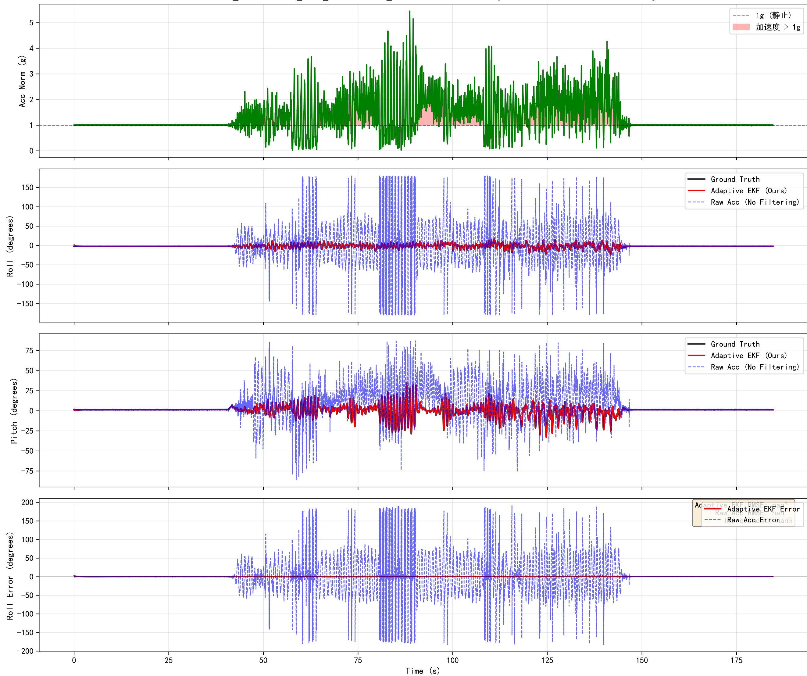
Scene: 15_undisturbed_fast_translation_A - Fast Motion Analysis (Inertial Frame Filtering)
