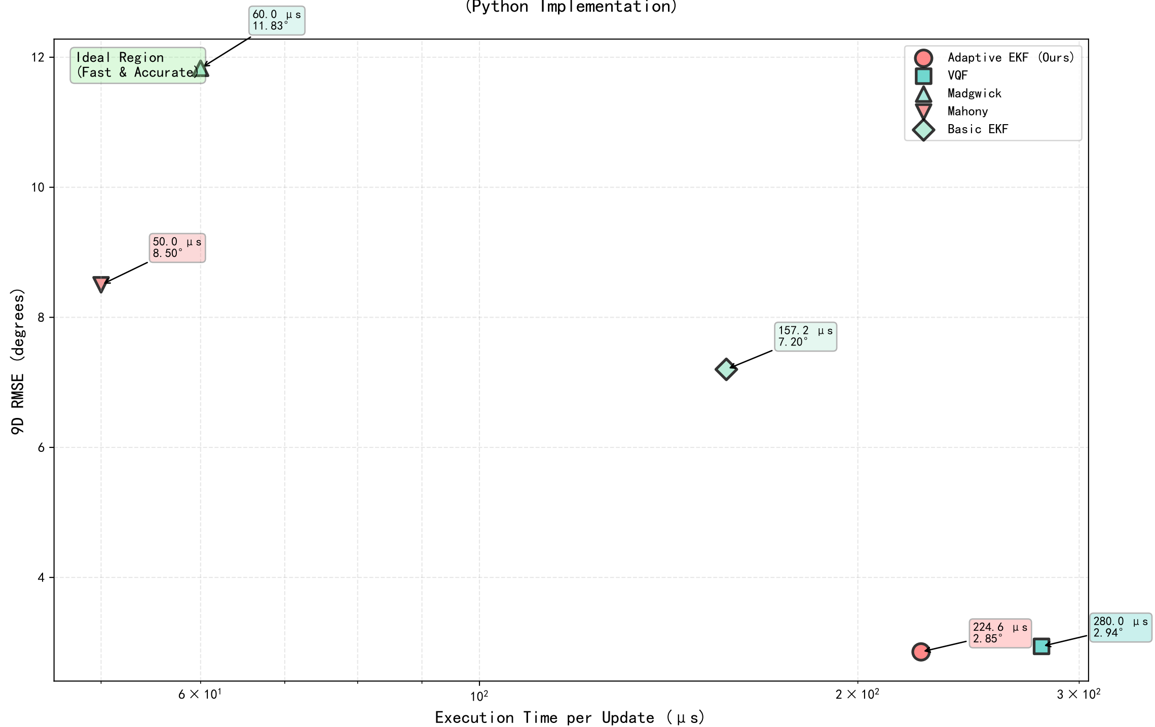
Computational Cost vs. Accuracy Trade-off (Python Implementation)
