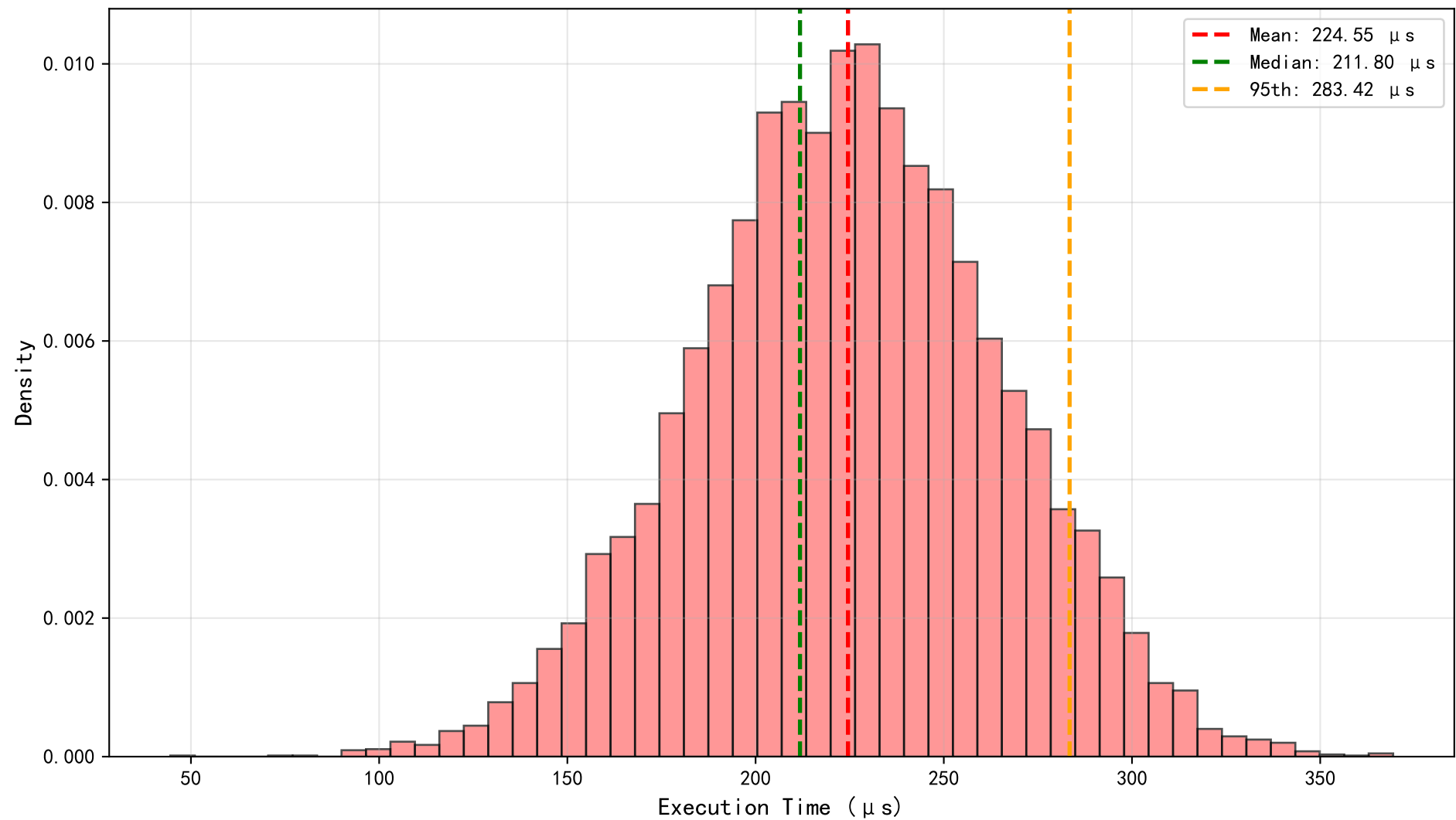
Execution Time Distribution (Adaptive EKF)
