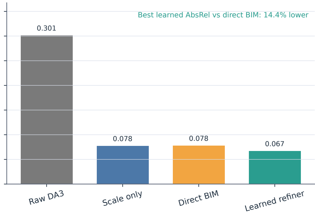
2D-3D-S Area 1
