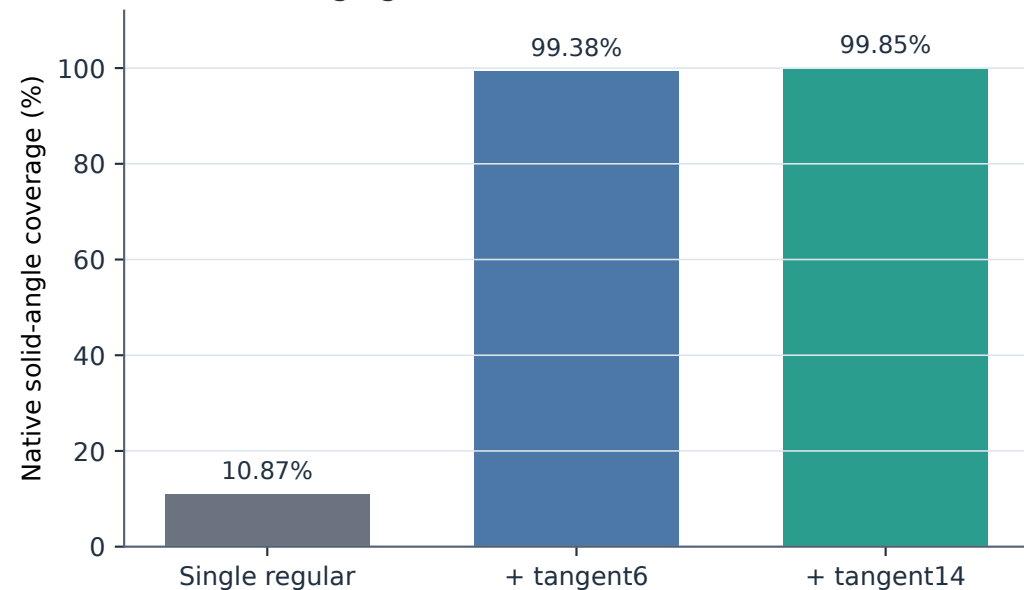
Coverage gain on each method's native union
