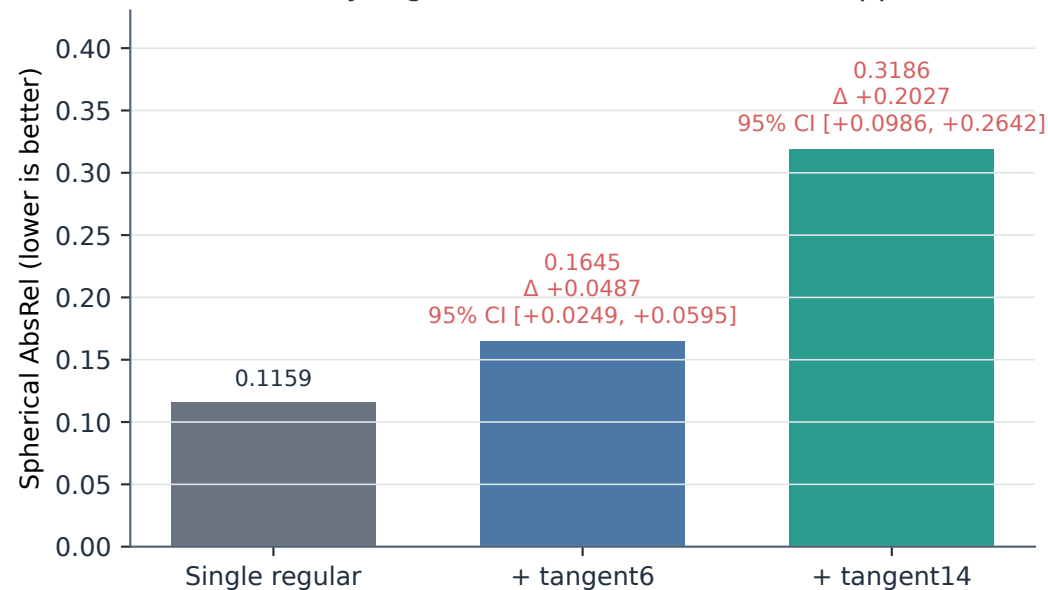
Accuracy regression on common strict support
