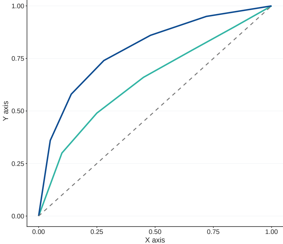
Calibration Curve (Binary Outcome)
