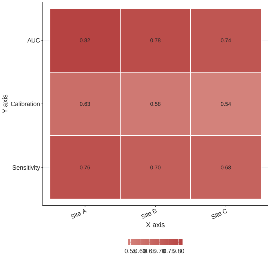
Heatmap (Group Comparison)
