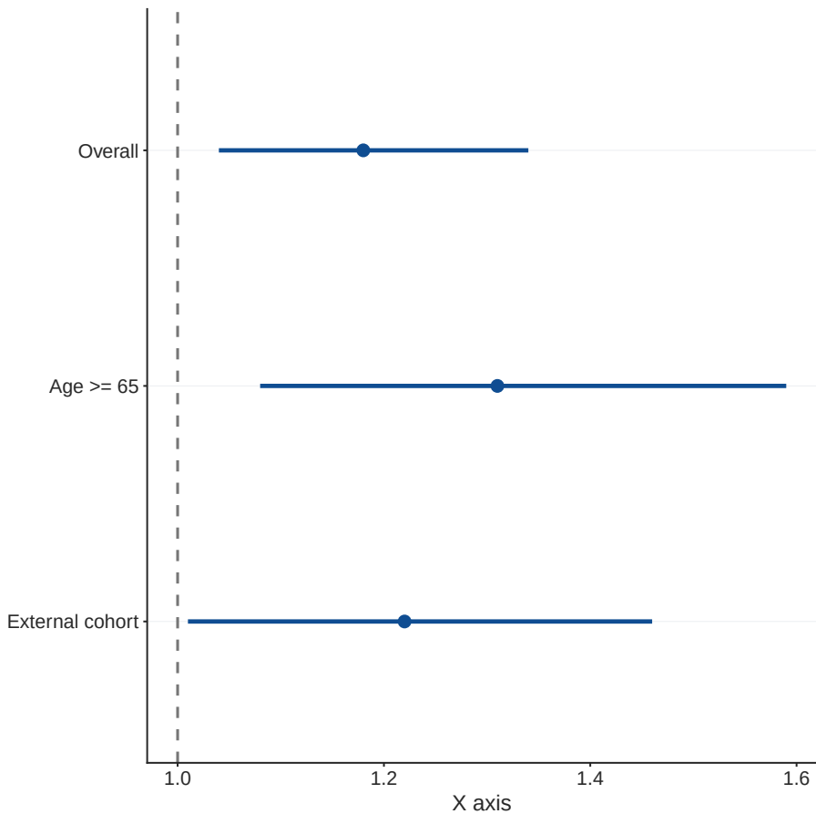
Forest Plot (Multivariable Model)
