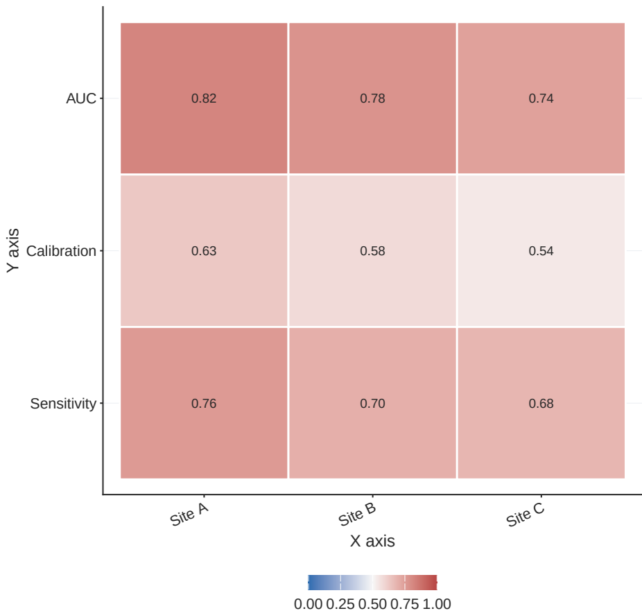
Performance Heatmap
