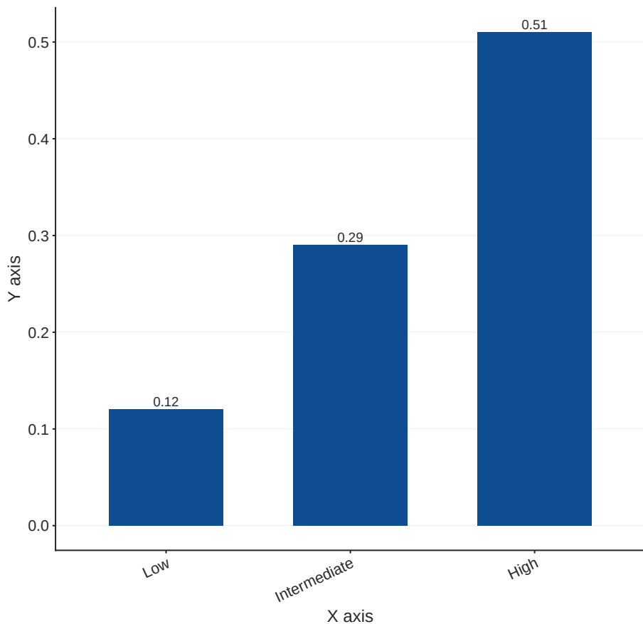
Risk-Group Summary (Time-to-Event)
