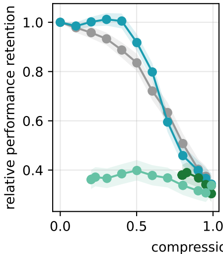
MATH-500
