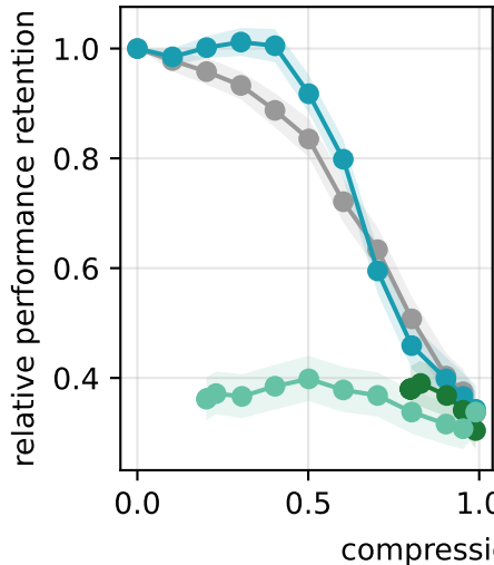
MATH-500
