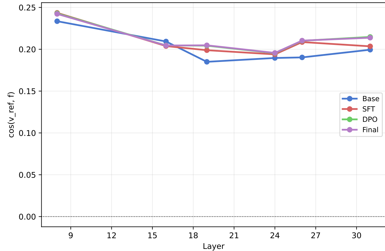
first generated token · logistic probe
