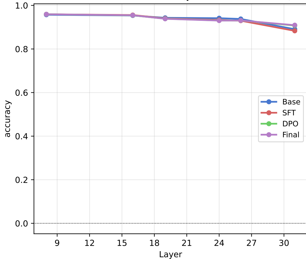
Probe acc — false refusal (pseudo vs harmless)
