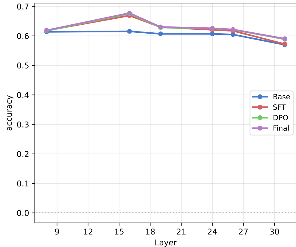
Probe acc — true refusal (harmful vs harmless)
