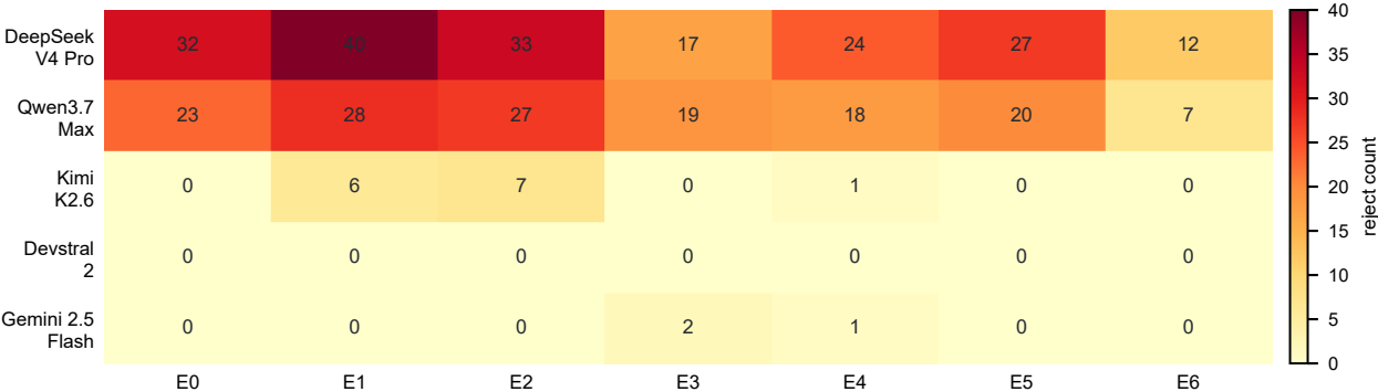
a Reject decisions per 98 packets; escalation dominates most cells
